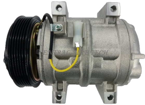
ZEXEL CAT NO. 46-002 COMPRESSOR TYPE: DKS15CH (4DM) CAR MODEL: S70 2.0/2.5L YEAR MODEL: 1998-1999 GROOVE: 6PK
