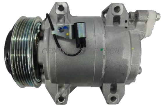
VALEO CAT NO. 46-004 COMPRESSOR TYPE: DKS17D CAR MODEL: S60 / XC90 2.5L YEAR MODEL: 2005 GROOVE: 6PK
