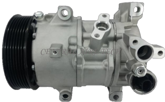
DENSO CAT NO. 44-152 COMPRESSOR TYPE: 6SES14C CAR MODEL: RAV 4 2.2L YEAR MODEL: 2014 GROOVE: 7PK
