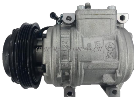
DENSO CAT NO. 44-082 COMPRESSOR TYPE: 10PA15L CAR MODEL: REVO 2.0L GAS YEAR MODEL: 2003 GROOVE: 4PK
