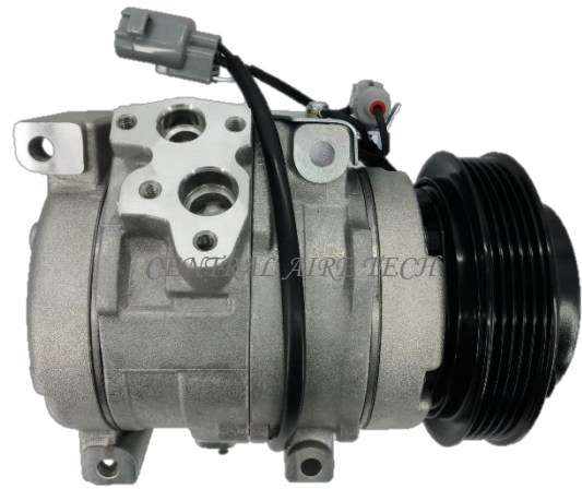
DENSO CAT NO. 44-133 COMPRESSOR TYPE: 10S15C (LSF) CAR MODEL: TOWNACE/LITE ACE YEAR MODEL: GROOVE: 5PK
