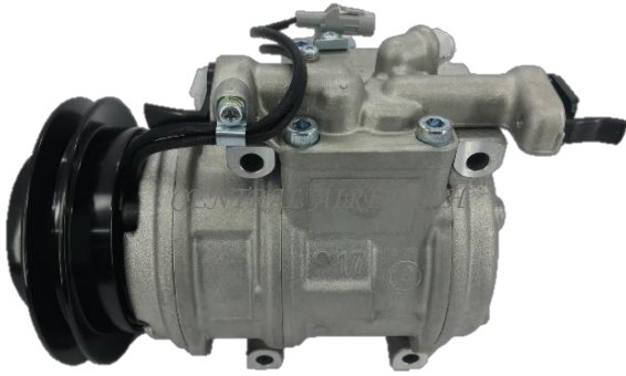
DENSO CAT NO. 44-083 COMPRESSOR TYPE: 10PA17C CAR MODEL: HI-ACE 2.0L DSL YEAR MODEL: 1997-2001 GROOVE: 1A
