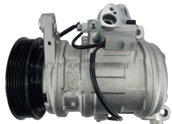
DENSO CAT NO. 44-094 COMPRESSOR TYPE: 10PA20H CAR MODEL: CROWN/LEXUS GS300 3.0L YEAR MODEL: 1997 GROOVE: 6PK
