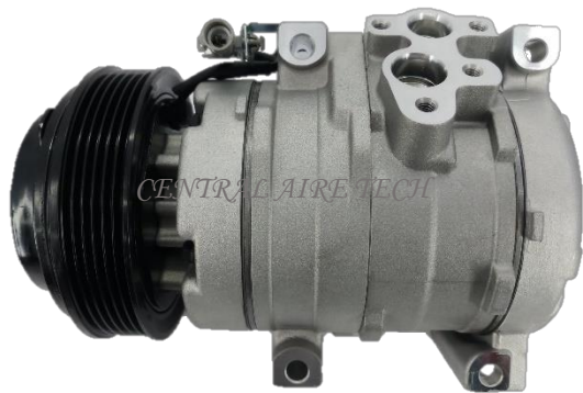
DENSO CAT NO. 44-097 COMPRESSOR TYPE: 10S15L CAR MODEL: ALTIS 1.6L YEAR MODEL: 2008 GROOVE: 6PK
