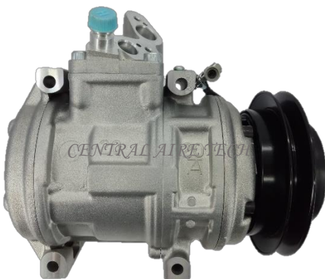
DENSO CAT NO. 44-093 COMPRESSOR TYPE: 10PA20C CAR MODEL: LAND CRUISER/PRADO YEAR MODEL: 1999 GROOVE: 1A
