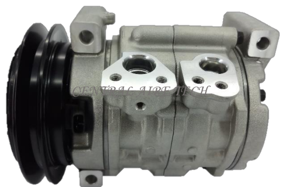
DENSO CAT NO. 44-137 COMPRESSOR TYPE: 10S11C (3DM) CAR MODEL: TOWNACE YEAR MODEL: GROOVE: 1A
