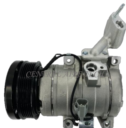
DENSO CAT NO. 44-024 COMPRESSOR TYPE: 10S17C CAR MODEL: EMINA YEAR MODEL: 2005 GROOVE: 6PK
