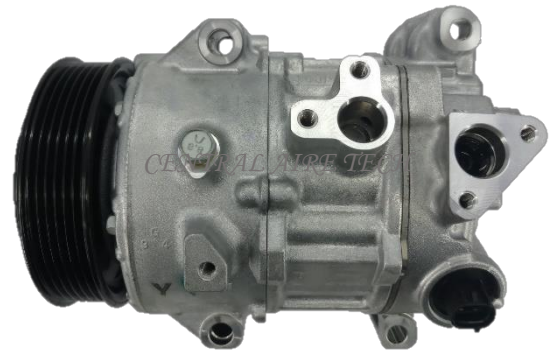
DENSO CAT NO. 44-074 COMPRESSOR TYPE: 7SES17C CAR MODEL: RAV 4 2.5L YEAR MODEL: 2015 GROOVE: 6PK
