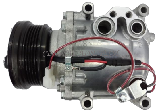
SANDEN CAT NO. 44-099 COMPRESSOR TYPE: TRF090 CAR MODEL: COROLLA 2063 1.5L YEAR MODEL: 1993 GROOVE: 5PK
