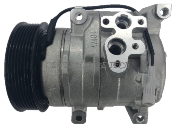
DENSO CAT NO. 44-016 COMPRESSOR TYPE: 10S15C CAR MODEL: INNOVA/FORTUNER GAS YEAR MODEL: 2005 GROOVE: 7PK
