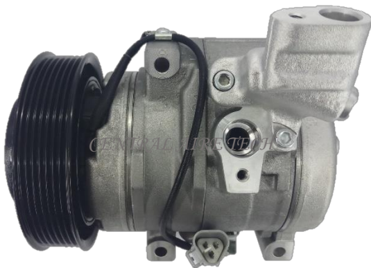
DENSO CAT NO. 44-015 COMPRESSOR TYPE: 10S15C CAR MODEL: RAV 4 2.0L YEAR MODEL: 2003 GROOVE: 7PK
