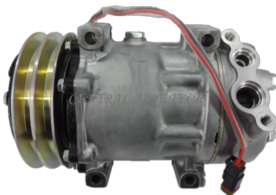
SANDEN CAT NO. 39-003 COMPRESSOR TYPE: SD7H15 (WK) CAR MODEL: SCANIA TRUCK 144 YEAR MODEL: GROOVE: 2A
