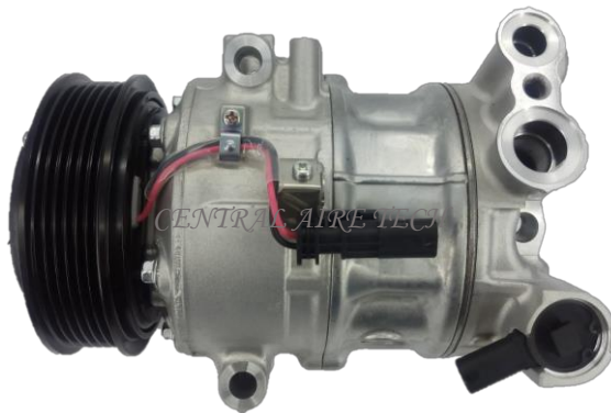
SANDEN CAT NO. 33-023 COMPRESSOR TYPE: PXC14 CAR MODEL: ASTRA/ANTARA YEAR MODEL: 2016 GROOVE: 6PK
