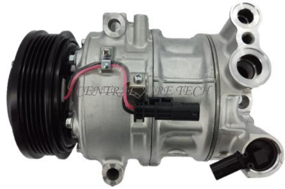
SANDEN CAT NO. 33-020 COMPRESSOR TYPE: PXC14 CAR MODEL: ASTRA K 1.4 YEAR MODEL: 2016 GROOVE: 5PK
