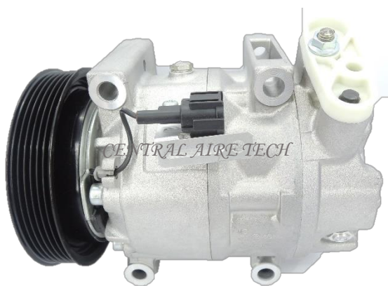
CALSONIC CAT NO. 32-001 COMPRESSOR TYPE: CWV618 (BH) CAR MODEL: CEFIRO 2.0L YEAR MODEL: 1997-2005 GROOVE: 6PK
