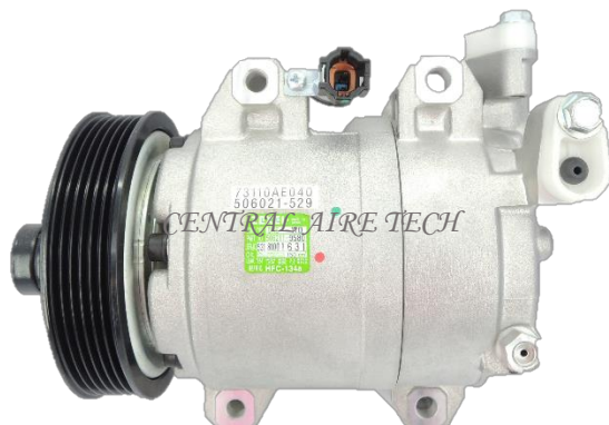
VALEO CAT NO. 32-041 COMPRESSOR TYPE: DKS17D CAR MODEL: MURANO 2.0L YEAR MODEL: 2006 GROOVE: 6PK
