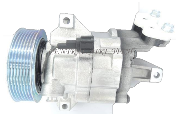
ZEXEL CAT NO. 32-018 COMPRESSOR TYPE: DKV08R CAR MODEL: TIIDA 1.5L YEAR MODEL: 2007-2009 GROOVE: 7PK
