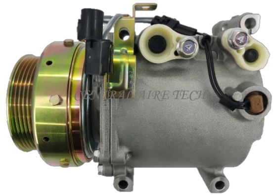
MITSUBISHI CAT NO. 31-002 COMPRESSOR TYPE: MSC90C CAR MODEL: GALANT 204G 2.0L YEAR MODEL: 1998 GROOVE: 5PK
