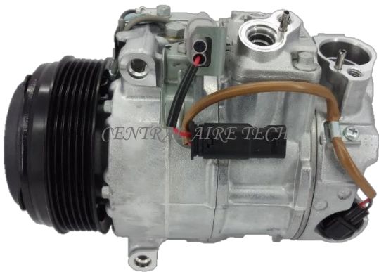
DENSO CAT NO. 29-069 COMPRESSOR TYPE: 6SBU16C CAR MODEL: W204 / C204 / W212 YEAR MODEL: 2007-2013 GROOVE: 6PK
