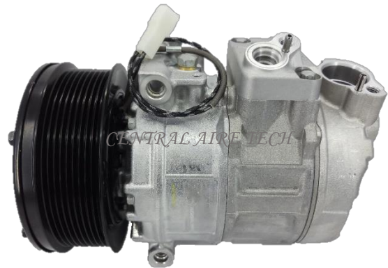
DENSO CAT NO. 29-070 COMPRESSOR TYPE: 7SBU16C CAR MODEL: ACTROSS MP2/MP3 YEAR MODEL: GROOVE: 9PK
