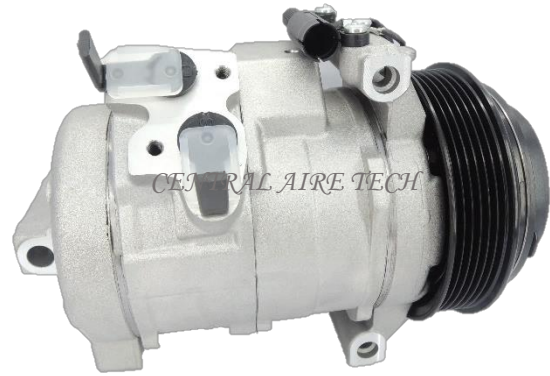
DENSO CAT NO. 29-026 COMPRESSOR TYPE: 10S17C CAR MODEL: SPRINTER 2500 / 3500 YEAR MODEL: 2007-2011 GROOVE: 6PK
