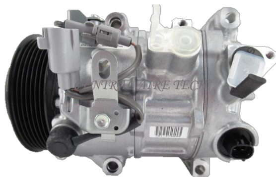
DENSO CAT NO. 27-012 COMPRESSOR TYPE: 7SAS17C CAR MODEL: RX350 3.5L GAS YEAR MODEL: 2018 GROOVE: 7PK
