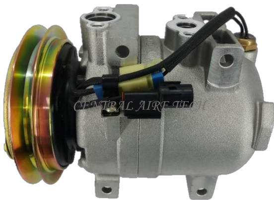
CALSONIC CAT NO. 26-003 COMPRESSOR TYPE: DKV14C CAR MODEL: BACK HOE YEAR MODEL: GROOVE: 1A
