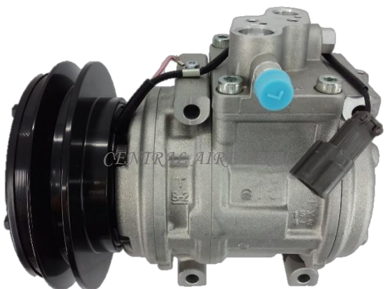
DENSO CAT NO. 26-006 COMPRESSOR TYPE: 10PA15C CAR MODEL: KOMATSU EXCAVATOR YEAR MODEL: 2008 GROOVE: 1B
