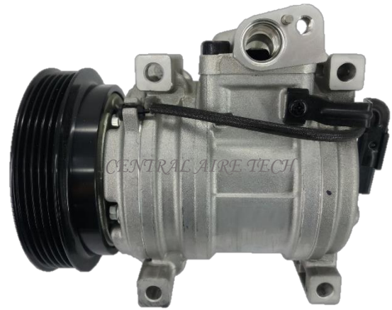
HALLA CAT NO. 24-002 COMPRESSOR TYPE: HS09 (4DM) CAR MODEL: PICANTO 1.0L YEAR MODEL: 2011 GROOVE: 5PK
