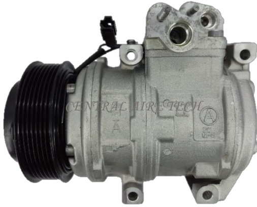
DOOWON CAT NO. 24-013 COMPRESSOR TYPE: 10PA17C CAR MODEL: SORENTO 2.0L YEAR MODEL: 2005 GROOVE: 7PK
