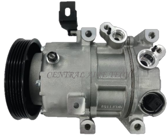
HANON CAT NO. 24-052 COMPRESSOR TYPE: VS16E (4DM) CAR MODEL: CARENS DSL YEAR MODEL: 2014 GROOVE: 5PK
