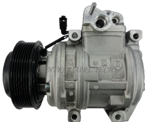
DOOWON CAT NO. 24-017 COMPRESSOR TYPE: 10PA15L CAR MODEL: SORENTO 2.5L DSL YEAR MODEL: 2008 GROOVE: 7PK
