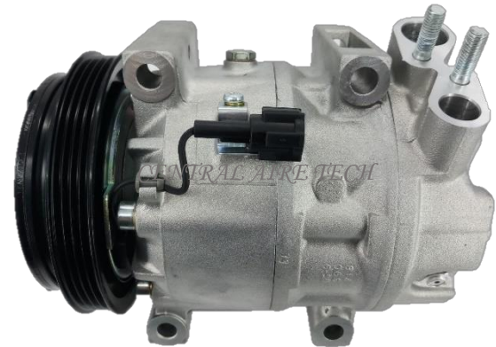
CALSONIC CAT NO. 21-010 COMPRESSOR TYPE: CWV618 CAR MODEL : QX4 BASE 3.5L YEAR MODEL: 2001-2003 GROOVE: 4PK
