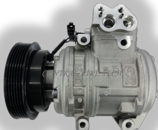
DOOWON CAT NO. 20-030 COMPRESSOR TYPE: 10PA15L (4DM INNER) CAR MODEL: TUCSON 2.0L DSL YEAR MODEL: 2008 GROOVE: 6PK
