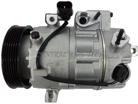
HALLA CAT NO. 20-061 COMPRESSOR TYPE: VS18E (3DM) CAR MODEL: SANTA FE/TUCSON YEAR MODEL: 2014 GROOVE: 6PK
