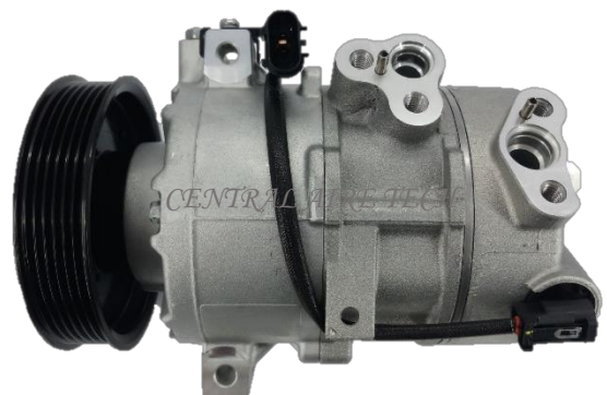
DOOWON CAT NO. 20-102 COMPRESSOR TYPE: DVE16N (SH) CAR MODEL: TUCSON YEAR MODEL: 2016 GROOVE: 6PK
