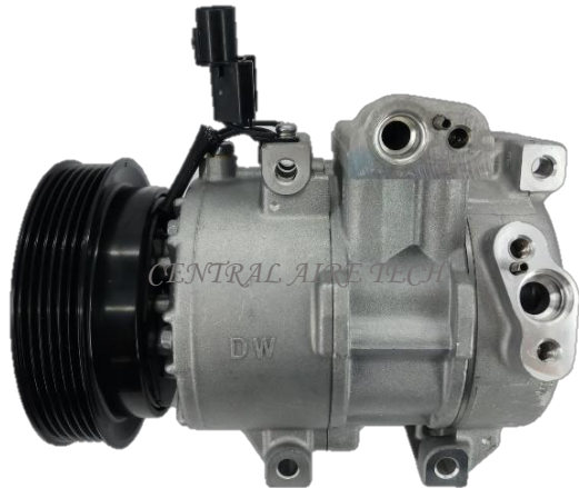
DOOWON CAT NO. 20-033 COMPRESSOR TYPE: DV12 (RSF) CAR MODEL: ACCENT 1.4L YEAR MODEL: 2012 GROOVE: 6PK
