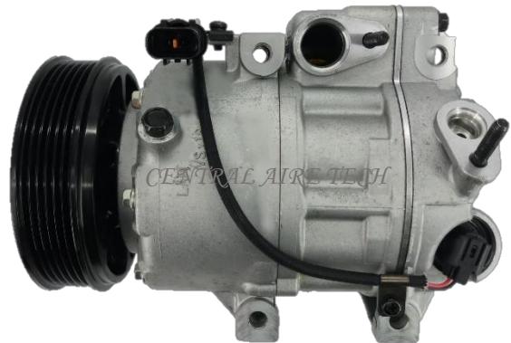
HALLA CAT NO. 20-022 COMPRESSOR TYPE: VS18E CAR MODEL: GENESIS 3.8L YEAR MODEL: 2010 GROOVE: 6PK
