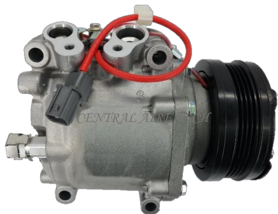
SANDEN CAT NO. 18-060 COMPRESSOR TYPE: TRS090 CAR MODEL: CIVIC 3067 2.0L/3061 1.3L YEAR MODEL: 1997 GROOVE: 4PK
