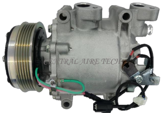
SANDEN CAT NO. 18-015 COMPRESSOR TYPE: TRSE07 CAR MODEL: JAZZ 3481 YEAR MODEL: 2012 GROOVE: 5PK
