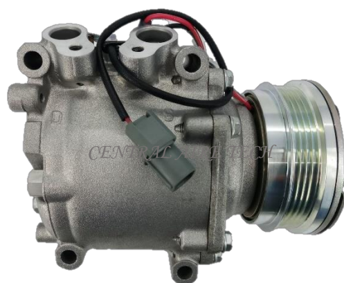
SANDEN CAT NO. 18-068 COMPRESSOR TYPE: TRS090 CAR MODEL : CIVIC 3058 1.5L YEAR MODEL: 1995 GROOVE: 4PK
