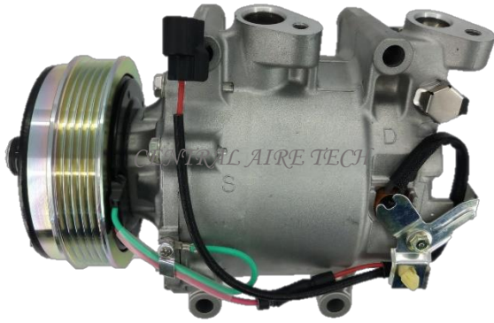
SANDEN CAT NO. 18-013 COMPRESSOR TYPE: TRSE07 CAR MODEL: JAZZ/CITY 3407/3423 1.5L YEAR MODEL: 2008 GROOVE: 5PK
