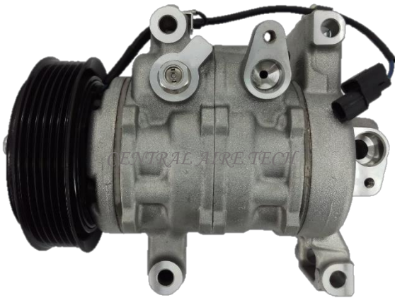
DENSO CAT NO. 18-057 COMPRESSOR TYPE: 10SRE11C CAR MODEL: FIT (USA) YEAR MODEL: 2015-2016 GROOVE: 6PK
