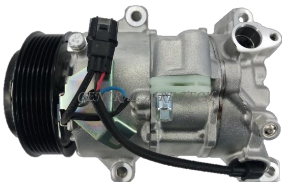
DENSO CAT NO. 18-087 COMPRESSOR TYPE: 6SAS14C CAR MODEL: STEPWAGON YEAR MODEL: 2015 GROOVE: 7PK
