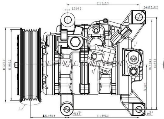
DENSO CAT NO. 18-058 COMPRESSOR TYPE: 10SRE13C CAR MODEL: MOBILIO 1.5L DSL YEAR MODEL: GROOVE: 7PK
