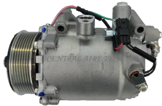
SANDEN CAT NO. 18-016 COMPRESSOR TYPE: TRSE09 CAR MODEL: CRV 37533 2.4L YEAR MODEL: 2008 GROOVE: 7PK
