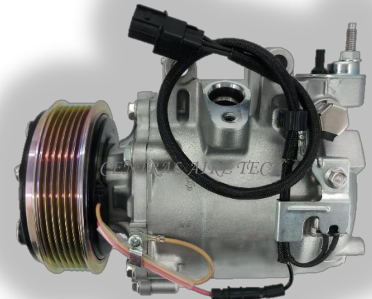
SANDEN CAT NO. 18-018 COMPRESSOR TYPE: TRSE09 CAR MODEL: CRV 3771 2.0L YEAR MODEL: 2012 GROOVE: 6PK
