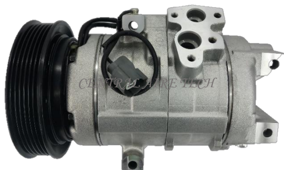
DENSO CAT NO. 18-033 COMPRESSOR TYPE: 10S20C (2DM REAR) CAR MODEL: ACCORD 3.0L YEAR MODEL: 2003 GROOVE: 6PK
