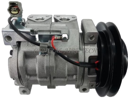
DENSO CAT NO. 16-001 COMPRESSOR TYPE: 10S13C CAR MODEL: RANGER YEAR MODEL: 2003-2011 GROOVE: 1A
