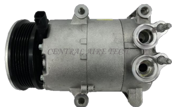
HALLA CAT NO. 14-011 COMPRESSOR TYPE: VS16 CAR MODEL: MONDEO 4 YEAR MODEL: 2012 GROOVE: 6PK
