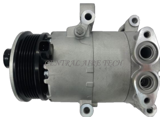
HALLA CAT NO. 14-008 COMPRESSOR TYPE: VS16 CAR MODEL: FOCUS 1.6L YEAR MODEL: 2005-2008 GROOVE: 6PK
