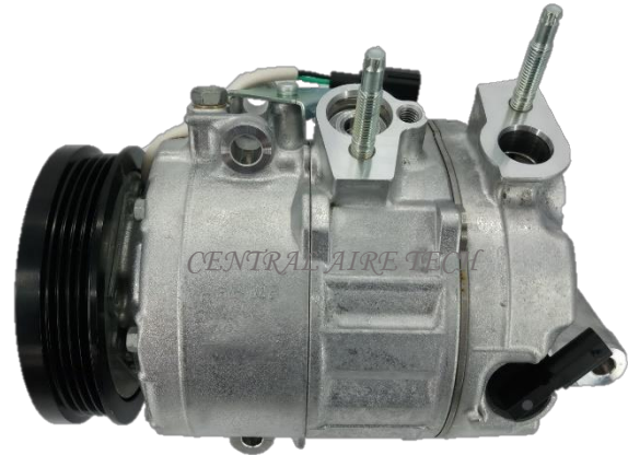
DENSO CAT NO. 14-094 COMPRESSOR TYPE: 7SAS17C CAR MODEL : FOCUS ST 2.3 ECOBOOST YEAR MODEL: GROOVE: 4PK
