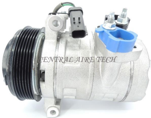
VALEO CAT NO. 12-009 COMPRESSOR TYPE: DKS17DS (RSF) CAR MODEL: NITRO/JEEP WRANGLER 3.8 YEAR MODEL: 2007-2011 GROOVE: 6PK
