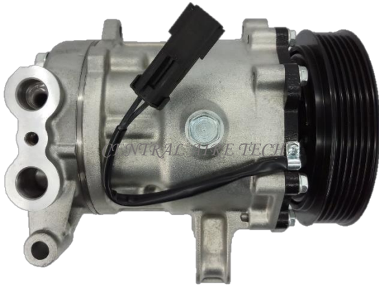
SANDEN CAT NO. 12-001 COMPRESSOR TYPE: SD7H15 (EM) CAR MODEL: DURANGO 4.7 YEAR MODEL: 2002 GROOVE: 6PK
