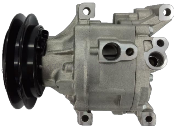
DENSO CAT NO. 11-009 COMPRESSOR TYPE: SCSA06C CAR MODEL: KUBOTA YEAR MODEL: 1999-2002 GROOVE: 1A
