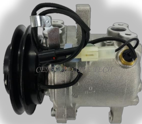
DENSO CAT NO. 11-006 COMPRESSOR TYPE: SV07E (3EM) CAR MODEL: KUBOTA TRACTOR YEAR MODEL: GROOVE: 1A
