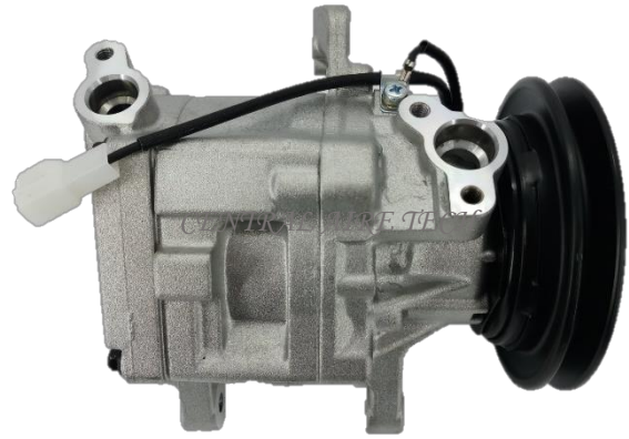
DENSO CAT NO. 11-008 COMPRESSOR TYPE: SC06E (3EM LSF) CAR MODEL: ATRAI/HIJET YEAR MODEL: 2000 GROOVE: 1A
