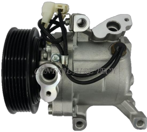
DENSO CAT NO. 11-001 COMPRESSOR TYPE: SV07C CAR MODEL: TERIOS 1.0/1.3L YEAR MODEL: 2007 GROOVE: 6PK
