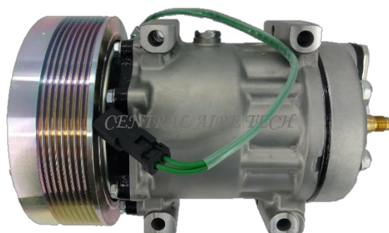
SANDEN CAT NO. 05-005 COMPRESSOR TYPE: SD7H15 (GK) CAR MODEL: CATERPILLAR 4840 YEAR MODEL: GROOVE: 8PK
