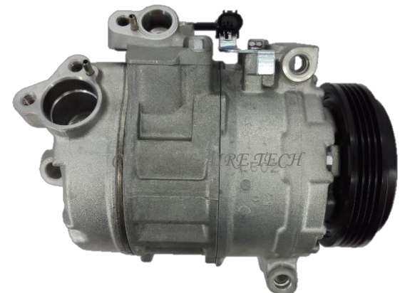
DENSO CAT NO. 02-036 COMPRESSOR TYPE: 7SEU17C CAR MODEL: 745i 4.4L YEAR MODEL: 2002-2005 GROOVE: 4PK
