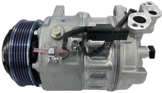
SANDEN CAT NO. 02-074 COMPRESSOR TYPE: PXC16 (EM) CAR MODEL: 540i 3.0L YEAR MODEL: 2017-2018 GROOVE: 6PK
