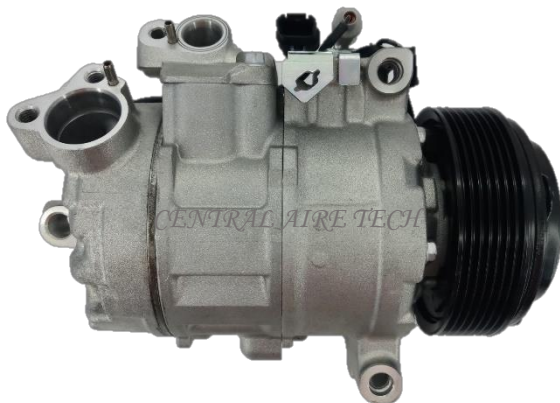
DENSO CAT NO. 02-065 COMPRESSOR TYPE: 6SBU14C (LSF 3DM) CAR MODEL: 5 SERIES/F11/F10 YEAR MODEL: 2009-2012 GROOVE: 7PK
