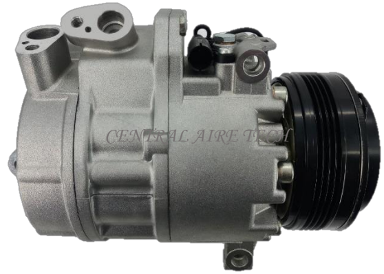
CALSONIC CAT NO. 02-014 COMPRESSOR TYPE: CSV717 CAR MODEL: X5 / E53 4.4L YEAR MODEL: 2004-2006 GROOVE: 4PK
