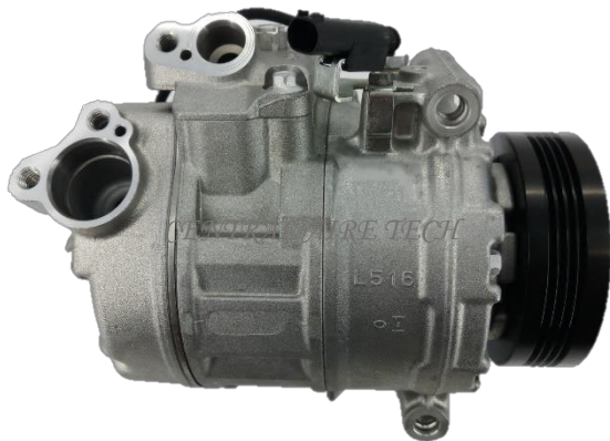
DENSO CAT NO. 02-009 COMPRESSOR TYPE: 7SEU17C CAR MODEL: E60 2.0/2.2/2.5 YEAR MODEL: 2003 GROOVE: 4PK
