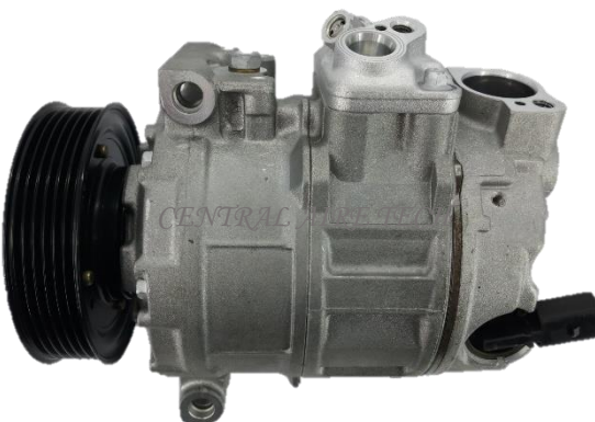
DENSO CAT NO. 01-005 COMPRESSOR TYPE: 7SEU16C CAR MODEL: A3 / GOLF 5 2.0L YEAR MODEL: 2006 GROOVE: 6PK
