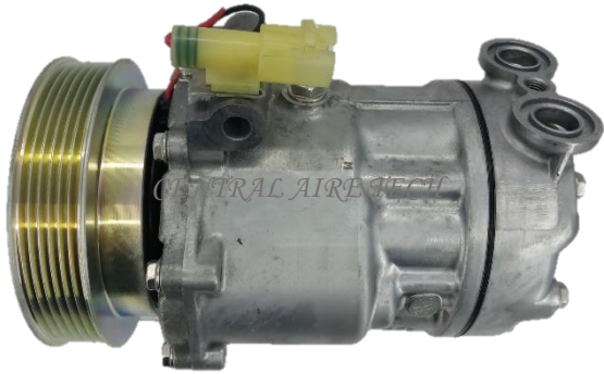
SANDEN CAT NO. 36-013 COMPRESSOR TYPE: SD7V16 (VSE) CAR MODEL: HATCHBACK 2.0L YEAR MODEL: 2000 GROOVE: 6PK
