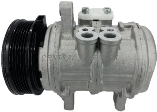
DENSO CAT NO. 14-103 COMPRESSOR TYPE: 6P148A (EM) CAR MODEL: MUSTANG GT 5.0L YEAR MODEL: 1982-1993 GROOVE: 6PK
