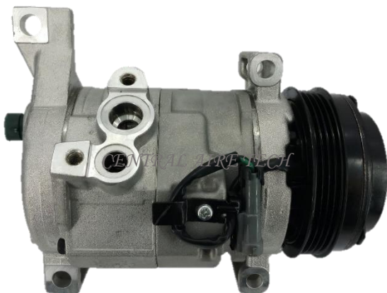
DENSO CAT NO. 07-017 COMPRESSOR TYPE: 10S17F CAR MODEL: SILVERADO YEAR MODEL: 2005 GROOVE: 4PK
