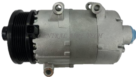
HALLA CAT NO. 14-009 COMPRESSOR TYPE: VS16 CAR MODEL: GALAXY 1.8 / 2.0L YEAR MODEL: 2005-2006 GROOVE: 6PK
