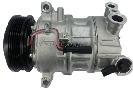
SANDEN CAT NO. 33-022 COMPRESSOR TYPE: PXC14 CAR MODEL: INSIGNIA 2.0T YEAR MODEL: 2017 GROOVE: 5PK
