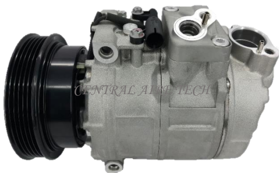
DENSO CAT NO. 36-005 COMPRESSOR TYPE: 7SBU16C CAR MODEL: RANGE ROVER YEAR MODEL: GROOVE: 5PK
