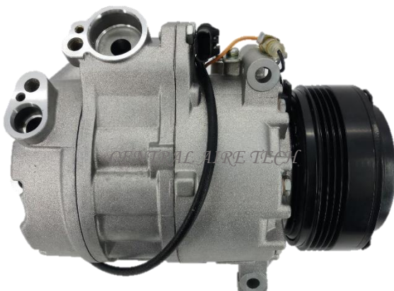
CALSONIC CAT NO. 02-023 COMPRESSOR TYPE: CSE717 CAR MODEL: X5 DSL 4.8 / E70 YEAR MODEL: 2006 GROOVE: 4PK
