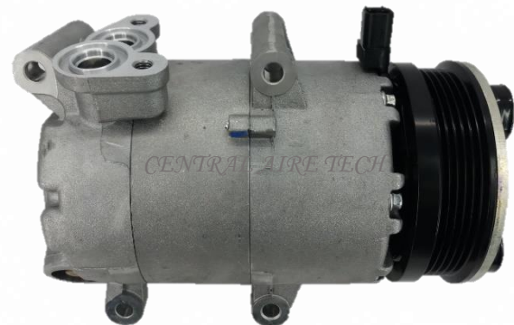
HALLA CAT NO. 14-018 COMPRESSOR TYPE: VS16 CAR MODEL: FOCUS 3.0L YEAR MODEL: 2012 GROOVE: 5PK
