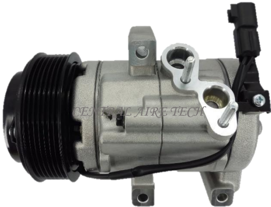
FOMOCO CAT NO. 14-051 COMPRESSOR TYPE: HS13N CAR MODEL: RANGER/MAZDA BT50 2.2L YEAR MODEL: 2012 GROOVE: 7PK
