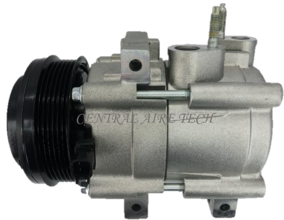
FOMOCO CAT NO. 14-002 COMPRESSOR TYPE: FS18 CAR MODEL: E150 5.4L YEAR MODEL: 2012 GROOVE: 6PK
