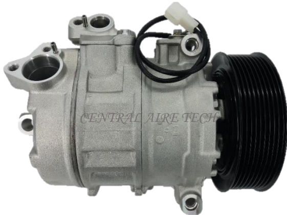
DENSO CAT NO. 29-039 COMPRESSOR TYPE: 7SBU16C CAR MODEL: ATEGO YEAR MODEL: 1999 GROOVE: 9PK
