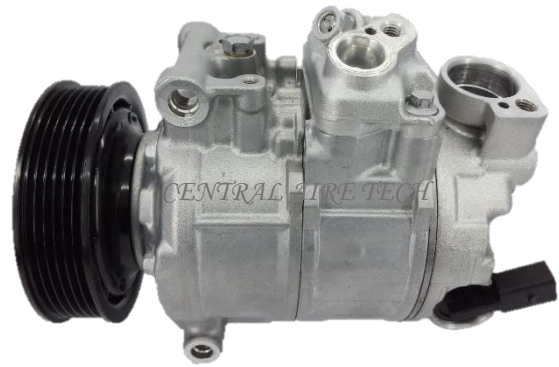
DENSO CAT NO. 01-016 COMPRESSOR TYPE: 6SEU14C CAR MODEL: Q3 YEAR MODEL: 2019 GROOVE: 6PK
