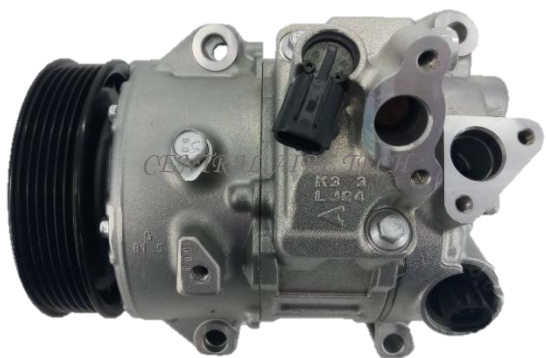
DENSO CAT NO. 44-168 COMPRESSOR TYPE: TSE17C CAR MODEL: CAMRY 2.5L YEAR MODEL: 2011 GROOVE: 6PK
