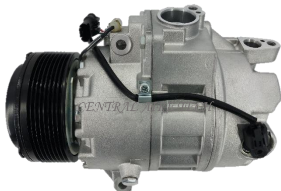
CALSONIC CAT NO. 02-024 COMPRESSOR TYPE: CSE717 CAR MODEL: X6 YEAR MODEL: 2008 GROOVE: 8PK
