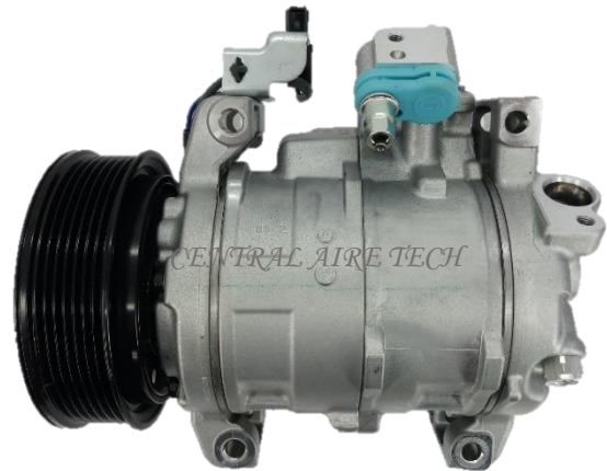
DENSO CAT NO. 18-088 COMPRESSOR TYPE: 10SRE20C CAR MODEL: ODYSSEY YEAR MODEL: 2014 GROOVE: 7PK
