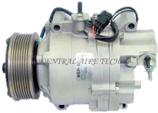
KEIHIN CAT NO. 18-025 COMPRESSOR TYPE: NSR-080 CAR MODEL: CIVIC YEAR MODEL: 2008 GROOVE: 7PK
