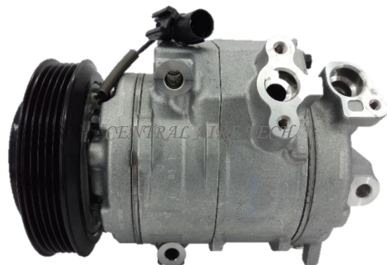
DENSO CAT NO. 31-060 COMPRESSOR TYPE: 10SRE15C CAR MODEL: XPANDER YEAR MODEL: 2018 GROOVE: 5PK
