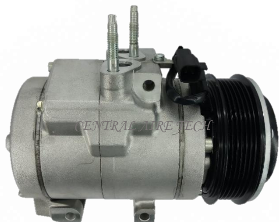
HALLA CAT NO. 14-042 COMPRESSOR TYPE: RS20 CAR MODEL: R250/F350 6.2L YEAR MODEL: 2011-2014 GROOVE: 6PK
