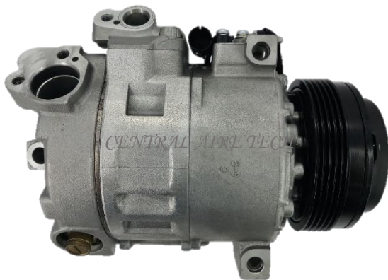
DENSO CAT NO. 02-063 COMPRESSOR TYPE: 7SB16C CAR MODEL: E39 YEAR MODEL: 1995-1997 GROOVE: 5PK
