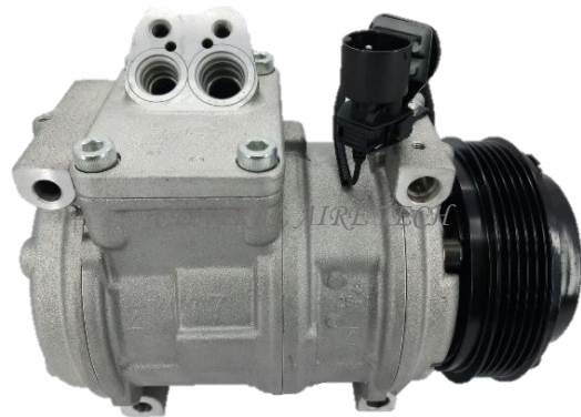
DENSO CAT NO. 02-058 COMPRESSOR TYPE: 10PA17C (LB) CAR MODEL: BMW 2.5/2.8/3.0L YEAR MODEL: 1991-1994 GROOVE: 5PK
