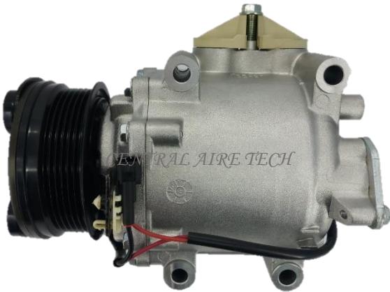
HALLA CAT NO. 14-027 COMPRESSOR TYPE: SC90V CAR MODEL: CROWN VICTORIA 4.6L YEAR MODEL: 2008 GROOVE: 6PK
