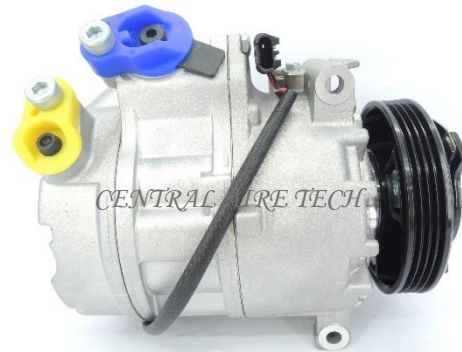
CALSONIC CAT NO. 02-028 COMPRESSOR TYPE: CSE717 CAR MODEL: X5 / X-DRIVE 4.4 / E70 YEAR MODEL: 2008 GROOVE: 4PK
