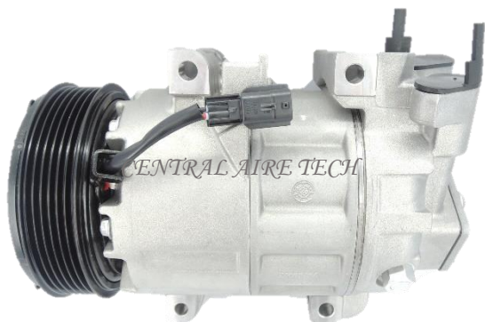
VALEO CAT NO. 32-067 COMPRESSOR TYPE: VCS14IC CAR MODEL: ALTIMA 2.5L YEAR MODEL: 2013-2017 GROOVE: 6PK
