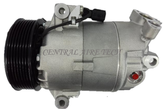
DELPHI CAT NO. 37-018 COMPRESSOR TYPE: 5CVC CAR MODEL: GRAND SCENIC 2.0L DCI YEAR MODEL: GROOVE: 7PK
