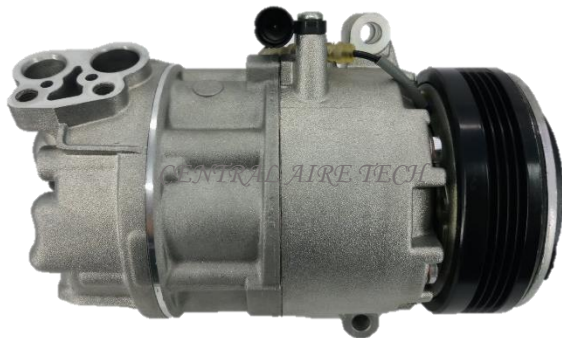
CALSONIC CAT NO. 02-021 COMPRESSOR TYPE: CSV613 CAR MODEL: E46 / E85 Z4 YEAR MODEL: 2003-2005 GROOVE: 4PK
