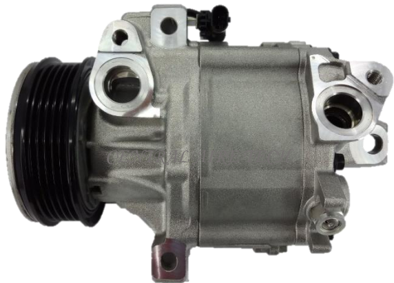
DENSO CAT NO. 07-064 COMPRESSOR TYPE: SCSE06C CAR MODEL: SPARK LS/LT/LTZ 1.4L YEAR MODEL: 2016-2021 GROOVE: 5PK
