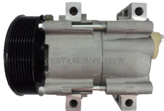
HALLA CAT NO. 14-102 COMPRESSOR TYPE: FS10 (BF) CAR MODEL : E150 YEAR MODEL: GROOVE: 8PK
