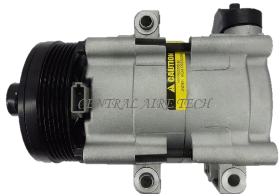
DENSO CAT NO. 14-066 COMPRESSOR TYPE: FS10 CAR MODEL: EXPLORER YEAR MODEL: GROOVE: 6PK
