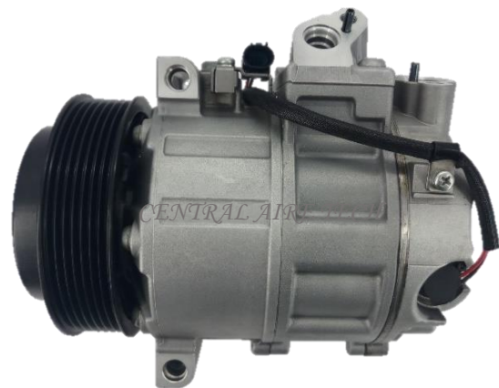
VALEO CAT NO. 29-028 COMPRESSOR TYPE: DCS17E CAR MODEL: W211 1.8L YEAR MODEL: 2008 GROOVE: 7PK
