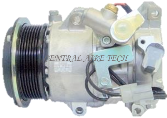
DENSO CAT NO. 44-031 COMPRESSOR TYPE: 6SEU16C CAR MODEL: HI ACE GAS YEAR MODEL: 2005 GROOVE: 7PK
