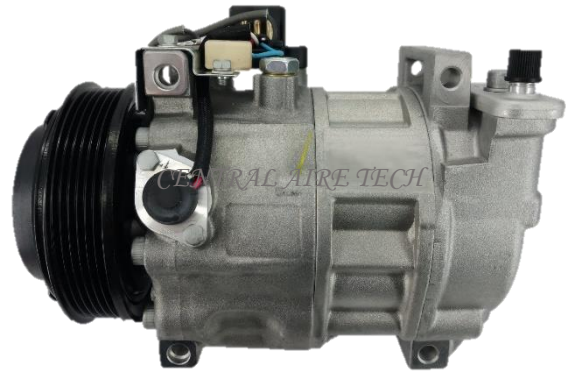
DENSO CAT NO. 29-014 COMPRESSOR TYPE: 6CA17C CAR MODEL: C220 2.2L YEAR MODEL: 1994 GROOVE: 6PK
