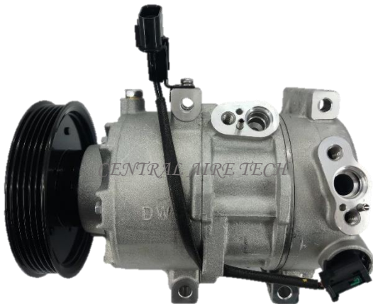
DOOWON CAT NO. 20-045 COMPRESSOR TYPE: DVE12 (4DM) CAR MODEL: ACCENT 1.4L YEAR MODEL: 2012 GROOVE: 5PK
