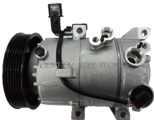
HALLA CAT NO. 20-057 COMPRESSOR TYPE: VS14E (4DM) CAR MODEL: ELANTRA/SOUL YEAR MODEL: 2014 GROOVE: 6PK
