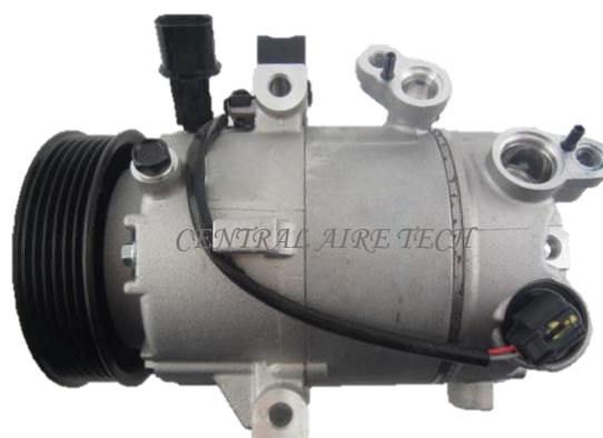
HALLA CAT NO. 20-058 COMPRESSOR TYPE: VS14E (3DM) CAR MODEL: ELANTRA 1.8L YEAR MODEL: 2015 GROOVE: 6PK
