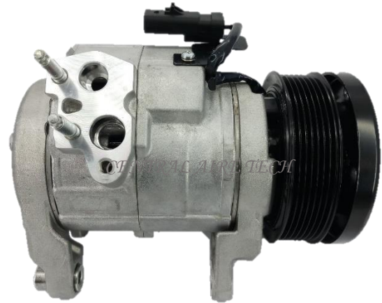
DENSO CAT NO. 12-004 COMPRESSOR TYPE: 10S20E CAR MODEL: DURANGO 3.7/4.7L YEAR MODEL: 2005 GROOVE: 7PK
