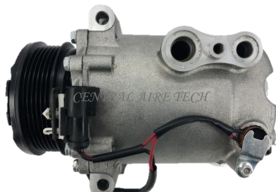
VISTEON CAT NO. 38-006 COMPRESSOR TYPE: SC90V CAR MODEL: SATURN VUE 3.5L YEAR MODEL: 2002 GROOVE: 6PK
