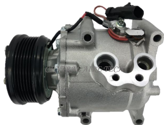
SANDEN CAT NO. 12-025 COMPRESSOR TYPE: TRSA09 CAR MODEL: STRATUS 2.4L YEAR MODEL: 2001-2003 GROOVE: 6PK
