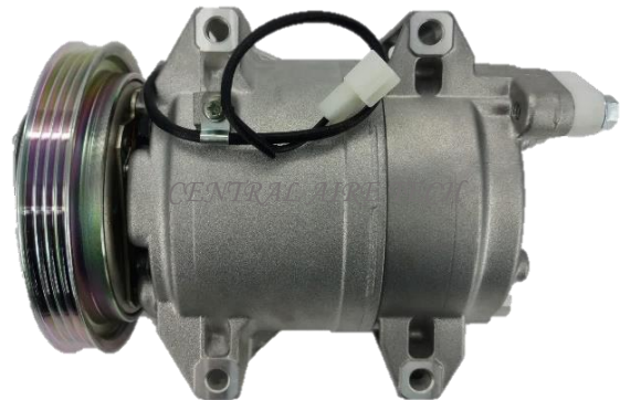
VALEO CAT NO. 32-088 COMPRESSOR TYPE: DKS17D CAR MODEL: VANETTE / MAZDA BONGO YEAR MODEL: 2007 GROOVE: 4PK
