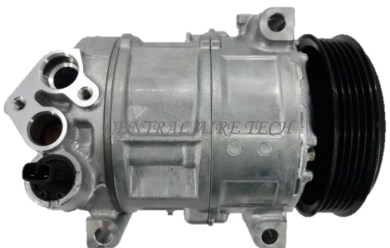
DENSO CAT NO. 13-011 COMPRESSOR TYPE: 5SL12C CAR MODEL: PUNTO 0.9L TURBO YEAR MODEL: GROOVE: 5PK
