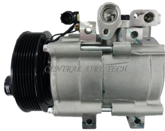
HALLA CAT NO. 20-008 COMPRESSOR TYPE: HS18 CAR MODEL : STAREX 2.5L YEAR MODEL: 2004 GROOVE: 7PK
