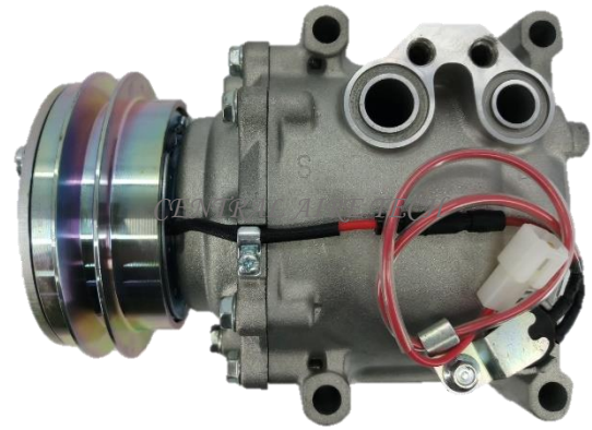
SANDEN CAT NO. 44-103 COMPRESSOR TYPE: TRS090 CAR MODEL: FX 3029 2.5L DSL YEAR MODEL: 1997 GROOVE: 1A
