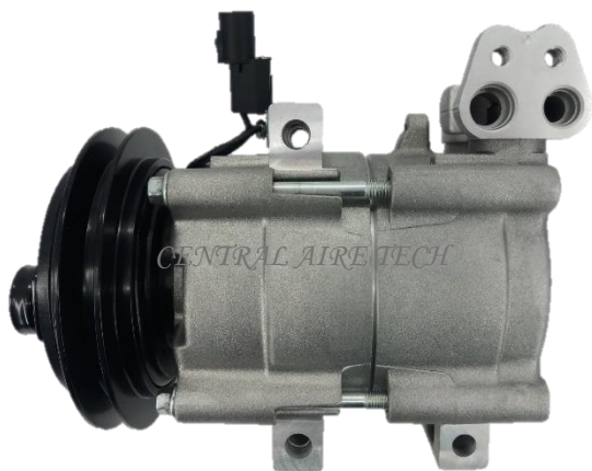
HALLA CAT NO. 20-067 COMPRESSOR TYPE: FS10 CAR MODEL: H100 / GALLOPER 2.5L YEAR MODEL: 1997 GROOVE: 1A
