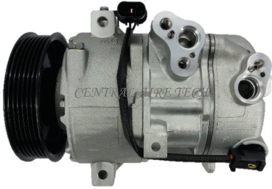
DOOWON CAT NO. 24-025 COMPRESSOR TYPE: DVE18 (3DM) CAR MODEL: SORENTO 2.2L YEAR MODEL: 2014 GROOVE: 6PK
