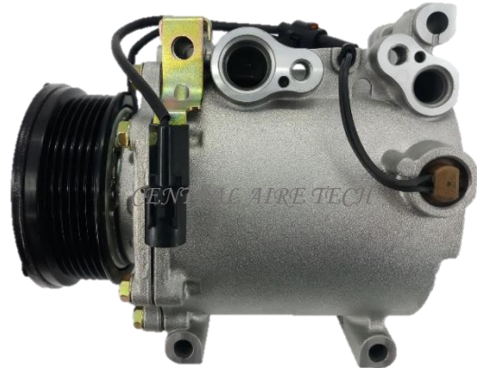
MITSUBISHI CAT NO. 31-088 COMPRESSOR TYPE: MSC90C CAR MODEL: OUTLANDER 215 1.6L YEAR MODEL: 2005 GROOVE: 6PK
