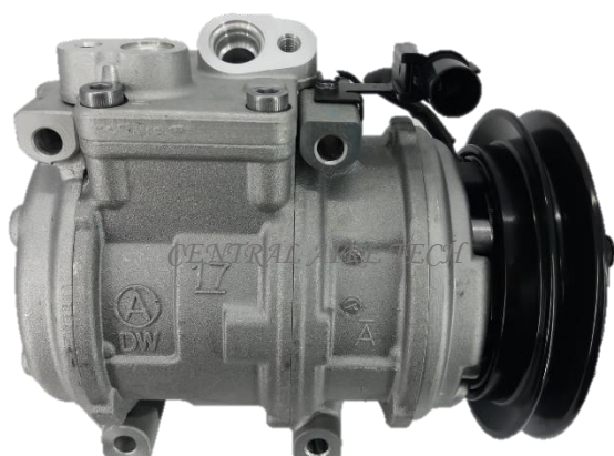
DOOWON CAT NO. 20-041 COMPRESSOR TYPE: 10PA17C CAR MODEL: COUNTY LH YEAR MODEL: 2012 GROOVE: 1A
