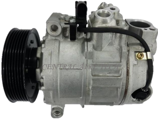
DENSO CAT NO. 01-007 COMPRESSOR TYPE: 7SEU16C CAR MODEL: A8 2.7/3.0L YEAR MODEL: 2008 GROOVE: 7PK
