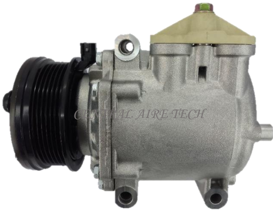
HALLA CAT NO. 14-025 COMPRESSOR TYPE: SC90V (RSF) CAR MODEL: EXPLORER 4.0L YEAR MODEL: 2005 GROOVE: 6PK
