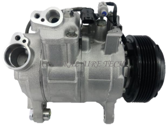
DENSO CAT NO. 02-062 COMPRESSOR TYPE: 6SBU14A (MF TYPE) CAR MODEL: Z4 2.0L YEAR MODEL: 2012 GROOVE: 6PK
