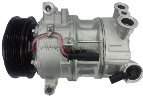
SANDEN CAT NO. 33-021 COMPRESSOR TYPE: PXC14 CAR MODEL: INSIGNIA 1.6 YEAR MODEL: 2016 GROOVE: 6PK
