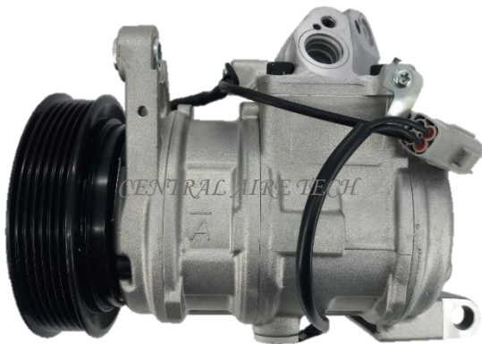
DENSO CAT NO. 44-091 COMPRESSOR TYPE: 10PA17H CAR MODEL: CROWN 2.0L YEAR MODEL: 1993-1994 GROOVE: 6PK
