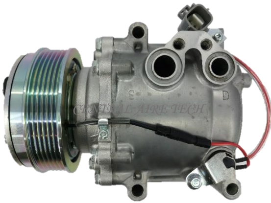
SANDEN CAT NO. 44-001 COMPRESSOR TYPE: TRS090 CAR MODEL: ALTIS 3102 1.3L YEAR MODEL: 2003 GROOVE: 6PK
