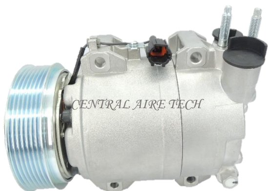
VALEO CAT NO. 32-049 COMPRESSOR TYPE: DKS17D CAR MODEL: URVAN E2.5 2.0L GAS YEAR MODEL: 2012 GROOVE: 7PK
