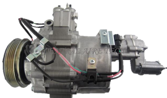
SANDEN CAT NO. 18-045 COMPRESSOR TYPE: HBC175 CAR MODEL: ACCORD HYBRID YEAR MODEL: 2006-2011 GROOVE: 4PK
