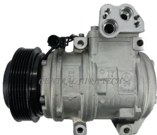
DOOWON CAT NO. 20-039 COMPRESSOR TYPE: 10PA17C CAR MODEL: GENESIS COUPE 2.0T L4 2L GAS YEAR MODEL: 2012 GROOVE: 6PK
