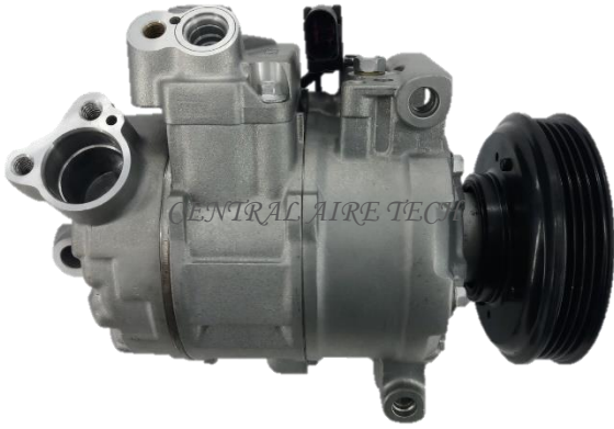
DENSO CAT NO. 01-013 COMPRESSOR TYPE: 6SEU14C (LSF) CAR MODEL: A4 1.9 YEAR MODEL: 2001 GROOVE: 4PK
