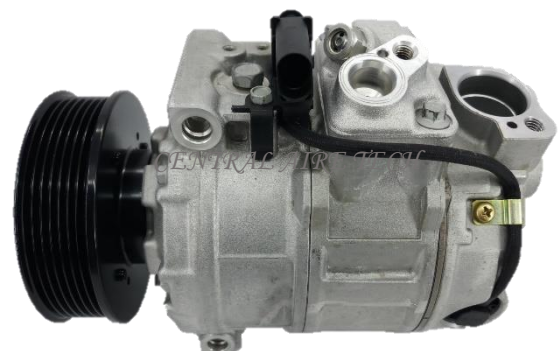
DENSO CAT NO. 45-036 COMPRESSOR TYPE: 7SEU16C CAR MODEL: TOUAREG 3.0L/3.6L V6 YEAR MODEL: 2009 GROOVE: 7PK
