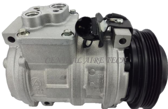
DENSO CAT NO. 02-059 COMPRESSOR TYPE: 10PA17C (SB) CAR MODEL: BMW 2.5/2.8/3.0L YEAR MODEL: 1991-1994 GROOVE: 4PK
