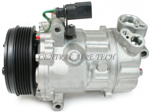
SANDEN CAT NO. 45-001 COMPRESSOR TYPE: SD6V12 (VGV) CAR MODEL: POLO DSL YEAR MODEL: 2001 GROOVE: 6PK
