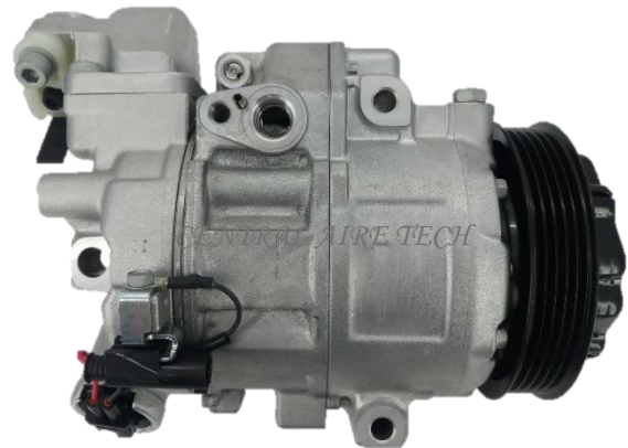
DENSO CAT NO. 29-080 COMPRESSOR TYPE: 6SEU12C CAR MODEL: A-CLASS A160/W168 1.6 YEAR MODEL: 2004 GROOVE: 5PK
