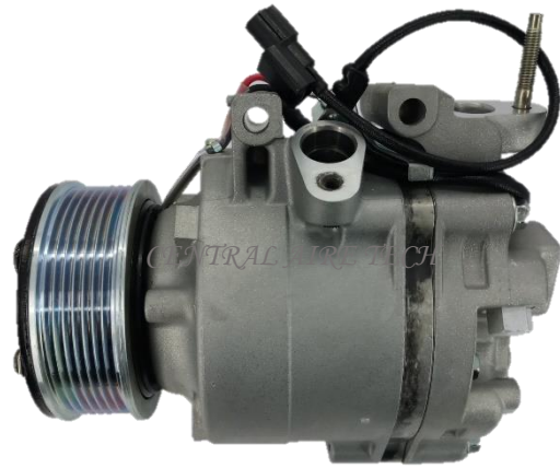
KEIHIN CAT NO. 18-026 COMPRESSOR TYPE: NSR-080 CAR MODEL : STREAM YEAR MODEL: 2006 GROOVE: 7PK
