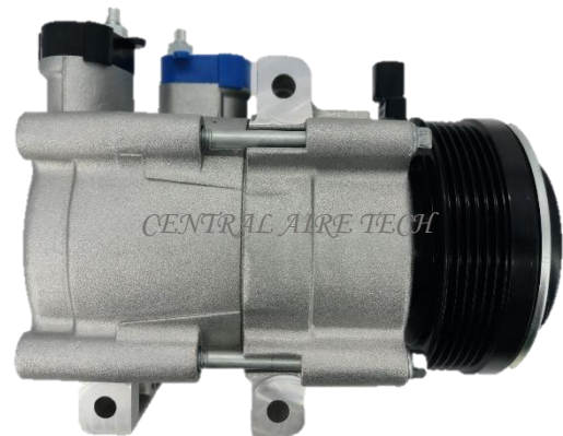
FOMOCO CAT NO. 14-084 COMPRESSOR TYPE: FS18 CAR MODEL: E150 5.4L YEAR MODEL: 2012 GROOVE: 6PK
