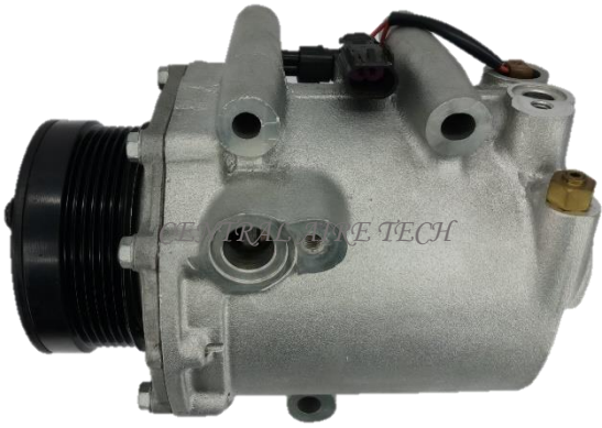
DELPHI CAT NO. 03-001 COMPRESSOR TYPE: MSC105CVSG4 CAR MODEL: RENDEZVOUS YEAR MODEL: 2002-2007 GROOVE: 6PK
