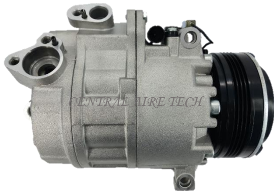
CALSONIC CAT NO. 02-069 COMPRESSOR TYPE: CSV717 (CENTER BH) CAR MODEL: X5 3.0 YEAR MODEL: 2002-2006 GROOVE: 4PK
