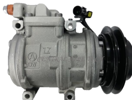
DOOWON CAT NO. 20-040 COMPRESSOR TYPE: 10PA17C CAR MODEL: COUNTY RH YEAR MODEL: 2012 GROOVE: 1A
