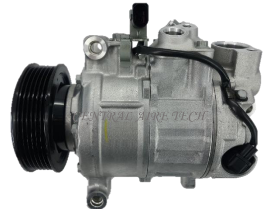
DENSO CAT NO. 01-011 COMPRESSOR TYPE: 6SEU14C CAR MODEL: A4 YEAR MODEL: 2003-2006 GROOVE: 6PK
