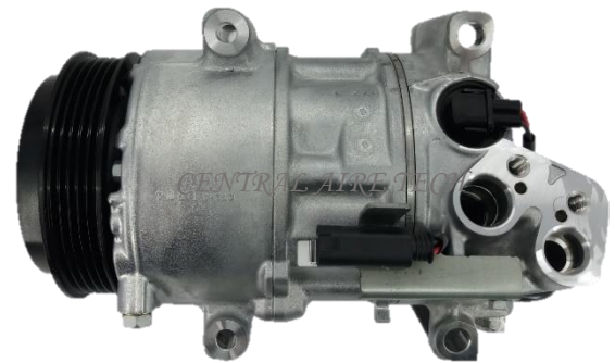
DENSO CAT NO. 29-016 COMPRESSOR TYPE: 6SEU16C CAR MODEL: B170 B-CLASS 2.0L YEAR MODEL: 2008 GROOVE: 5PK
