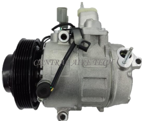
DENSO CAT NO. 27-011 COMPRESSOR TYPE: 7SBU16C CAR MODEL: SC430 4.3L YEAR MODEL: 2002-2010 GROOVE: 6PK
