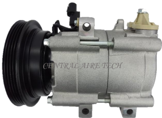
HALLA CAT NO. 32-087 COMPRESSOR TYPE: FS10 CAR MODEL: QUEST YEAR MODEL: GROOVE: 4PK
