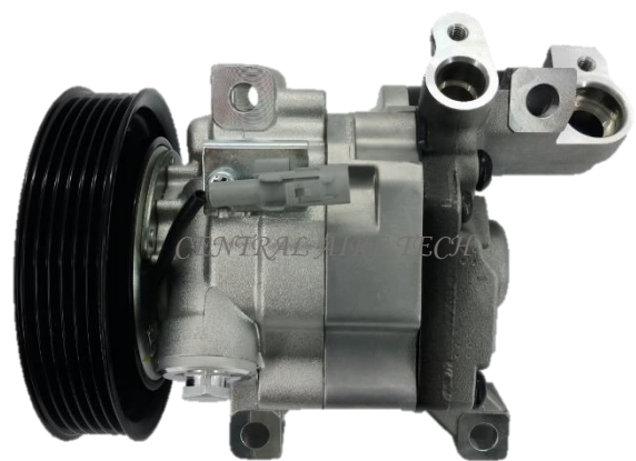
VALEO CAT NO. 34-006 COMPRESSOR TYPE: DKV06R (4DM) CAR MODEL: 107 1.4 YEAR MODEL: 2005-2014 GROOVE: 6PK
