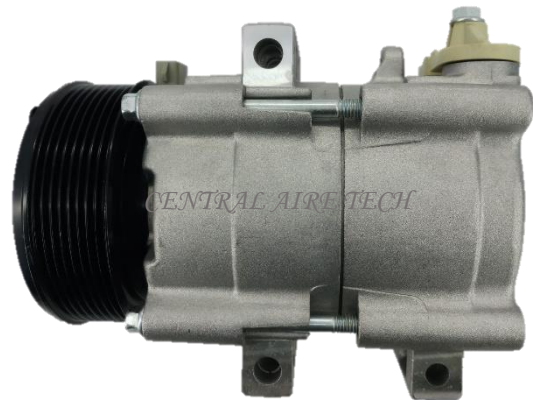
HALLA CAT NO. 14-082 COMPRESSOR TYPE: FS10 CAR MODEL: EXPEDITION 4.6L YEAR MODEL: 1999 GROOVE: 8PK
