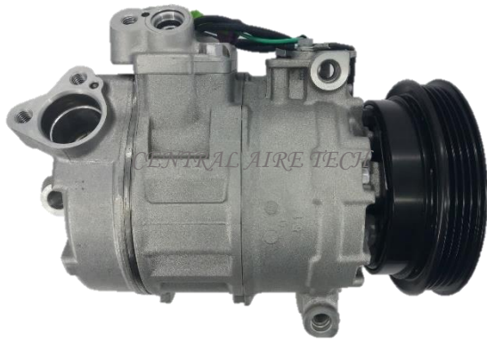
DENSO CAT NO. 45-013 COMPRESSOR TYPE: 7SBU16C CAR MODEL: PASSAT B5 YEAR MODEL: 2004 GROOVE: 4PK
