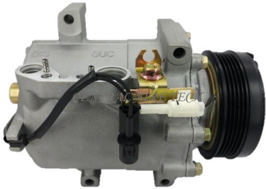
MITSUBISHI CAT NO. 12-020 COMPRESSOR TYPE: FX105VSL4 CAR MODEL: COLT BASE L4 1.5L YEAR MODEL: 1993 GROOVE: 5PK
