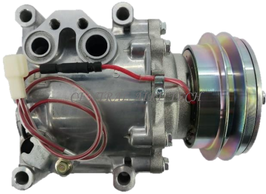
SANDEN CAT NO. 44-102 COMPRESSOR TYPE: TRS090 CAR MODEL: FX 3047/3088 2.0L GAS YEAR MODEL: 1997 GROOVE: 1A
