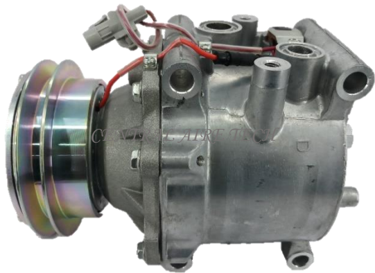
SANDEN CAT NO. 44-104 COMPRESSOR TYPE: TRS105 CAR MODEL: REVO 3215 2.0L DSL YEAR MODEL: 1999 GROOVE: 1A
