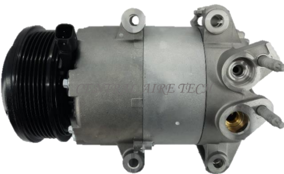
HALLA CAT NO. 14-017 COMPRESSOR TYPE: VS16 CAR MODEL: ECOSPORT 1.6L YEAR MODEL: 2012 GROOVE: 6PK
