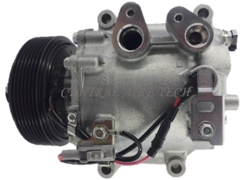
SANDEN CAT NO. 44-157 COMPRESSOR TYPE: TRSE09 CAR MODEL: TYT.INNOVA 3729 YEAR MODEL: 2017 GROOVE: 7PK
