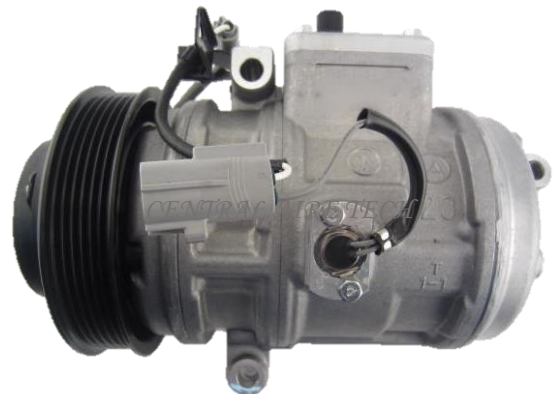
DENSO CAT NO. 44-092 COMPRESSOR TYPE: 10PA20C (3DM) CAR MODEL: LAND CRUISER 4.7L YEAR MODEL: 1999 GROOVE: 6PK
