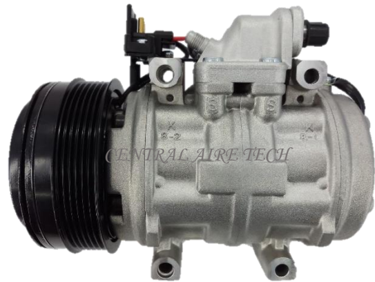
DENSO CAT NO. 29-040 COMPRESSOR TYPE: 10P15C CAR MODEL: W124 2.4L YEAR MODEL: 1989 GROOVE: 6PK
