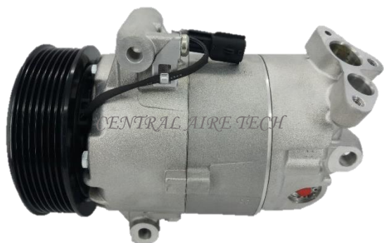
DELPHI CAT NO. 37-019 COMPRESSOR TYPE: 5CVC CAR MODEL: TRAFFIC YEAR MODEL: GROOVE: 7PK
