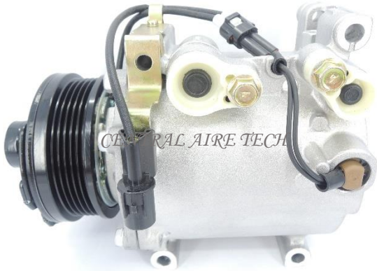
mitsubishi CAT NO. 31-001 COMPRESSOR TYPE: MSC90C CAR MODEL: LANCER 204N/204P 1.5L YEAR MODEL: 2003-2005 GROOVE: 5PK
