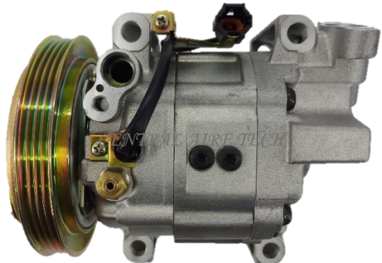
ZEXEL CAT NO. 32-114 COMPRESSOR TYPE: DKV14G (BH) CAR MODEL: SERIES 3 1.6L YEAR MODEL: 1997 GROOVE: 4PK
