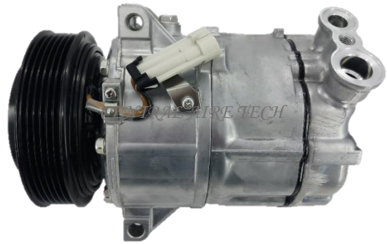
SANDEN CAT NO. 69-002 COMPRESSOR TYPE: PXV16 CAR MODEL: SAAB 9-3 AERO 2.8 YEAR MODEL: 2006-2009 GROOVE: 6PK
