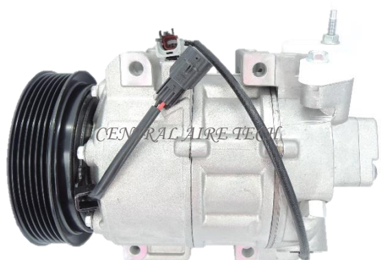
VALEO CAT NO. 32-057 COMPRESSOR TYPE: DCS17EC CAR MODEL: ALTIMA/X-TRAIL 2.5L YEAR MODEL: 2007-2010 GROOVE: 6PK
