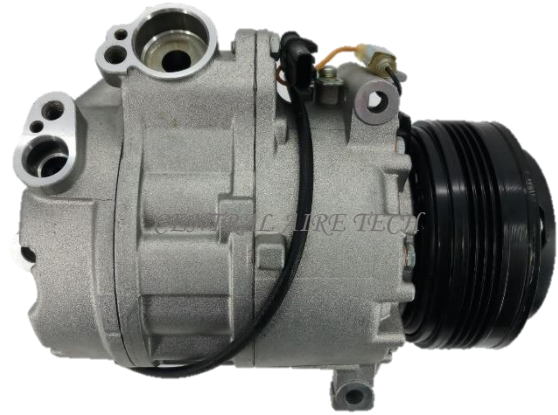
CALSONIC CAT NO. 02-026 COMPRESSOR TYPE: CSE717 CAR MODEL: X5 4.8L YEAR MODEL: 2008 GROOVE: 4PK
