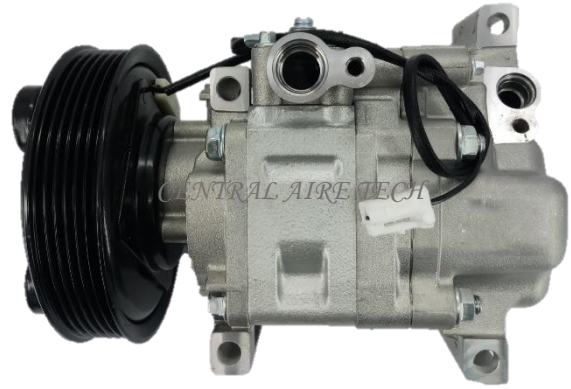
PANASONIC CAT NO. 28-002 COMPRESSOR TYPE: H12 (SH) CAR MODEL: MAZDA 3 1.6L YEAR MODEL: 2005 GROOVE: 6PK
