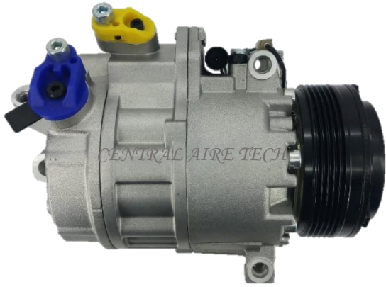
CALSONIC CAT NO. 02-067 COMPRESSOR TYPE: CSV717 (BH) CAR MODEL: X5 3.0 YEAR MODEL: 2006 GROOVE: 5PK
