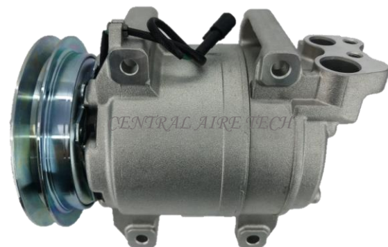
ZEXEL CAT NO. 22-105 COMPRESSOR TYPE: DKS15D CAR MODEL: ELF 5.2L YEAR MODEL: 2008 GROOVE: 1A
