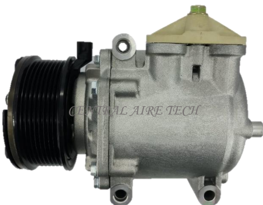
HALLA CAT NO. 14-065 COMPRESSOR TYPE: SC90V (RSF) CAR MODEL: EXPLORER YEAR MODEL: GROOVE: 8PK
