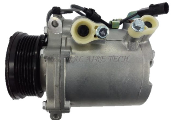
mitsubishi CAT NO. 31-006 COMPRESSOR TYPE: MSC90CAS CAR MODEL: OUTLANDER 221 2.4L YEAR MODEL: 2008 GROOVE: 6PK
