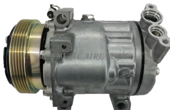
SANDEN CAT NO. 37-024 COMPRESSOR TYPE: SD7V16 (VPA) CAR MODEL: TWINGO 1.2L YEAR MODEL: 1999 GROOVE: 5PK
