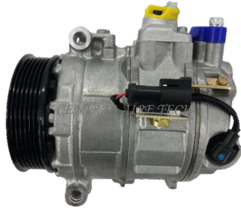
DENSO CAT NO. 36-008 COMPRESSOR TYPE: 7SEU17C CAR MODEL: DISCOVERY YEAR MODEL: 2004-2009 GROOVE: 6PK
