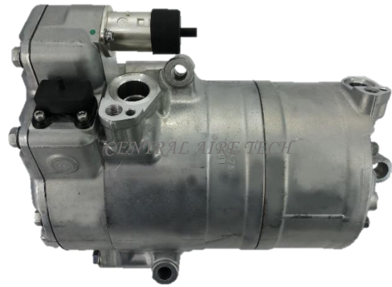
SANDEN CAT NO. 36-026 COMPRESSOR TYPE: SHS33 C.MODEL: RANGEROVER SPORT HYBRID YEAR MODEL: 2013 GROOVE: ELECTRIC
