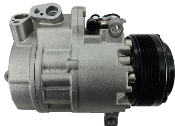
CALSONIC CAT NO. 02-012 COMPRESSOR TYPE: CSV717 CAR MODEL: X5 4.4/4.8 YEAR MODEL: 2006 GROOVE: 6PK
