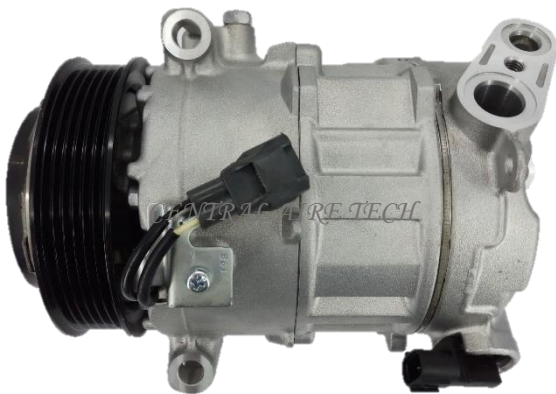
DENSO CAT NO. 06-011 COMPRESSOR TYPE: 7SBH17C CAR MODEL: JEEP CHEROKEE 3.2L YEAR MODEL: 2014-2020 GROOVE: 6PK
