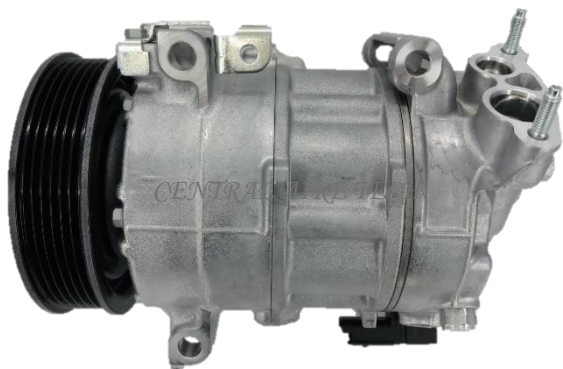
DENSO CAT NO. 34-013 COMPRESSOR TYPE: 6SEL16C CAR MODEL: 308 YEAR MODEL: GROOVE: 6PK
