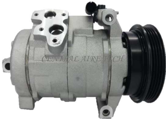
DENSO CAT NO. 45-015 COMPRESSOR TYPE: 10S17C CAR MODEL: CRAFTER 2.5L YEAR MODEL: 2006 GROOVE: 4PK
