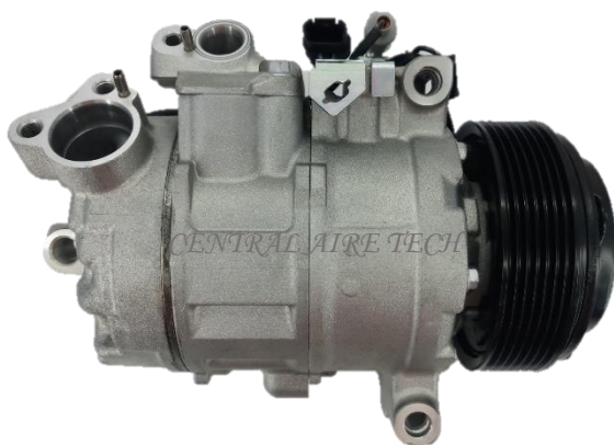
DENSO CAT NO. 02-065 COMPRESSOR TYPE: 6SBU14C (LSF 3DM) CAR MODEL: 5 SERIES/F11/F10 YEAR MODEL: 2009-2012 GROOVE: 7PK
