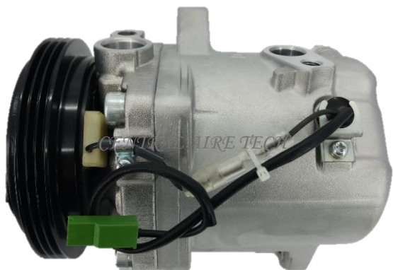
SEIKO SEIKI CAT NO. 40-001 COMPRESSOR TYPE: SS72DLG1 CAR MODEL: FORTWO 0.8L YEAR MODEL: 2004 GROOVE: 3PK
