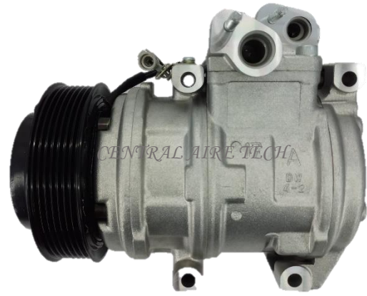
DOOWON CAT NO. 24-056 COMPRESSOR TYPE: 10PA17C CAR MODEL: SORENTO YEAR MODEL: GROOVE: 7PK
