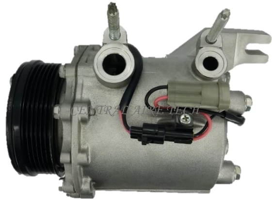
DELPHI CAT NO. 03-002 COMPRESSOR TYPE: MSC105CG2 CAR MODEL: UPLANDER YEAR MODEL: 2008 GROOVE: 6PK
