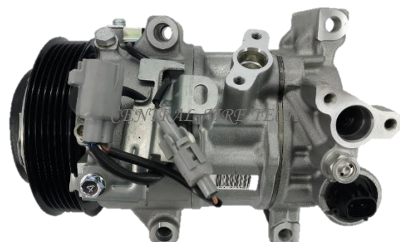
DENSO CAT NO. 44-179 COMPRESSOR TYPE: 6SAS14C CAR MODEL: COROLLA ECO/LE ECO 1.8L YEAR MODEL: 2015-2016 GROOVE: 6PK
