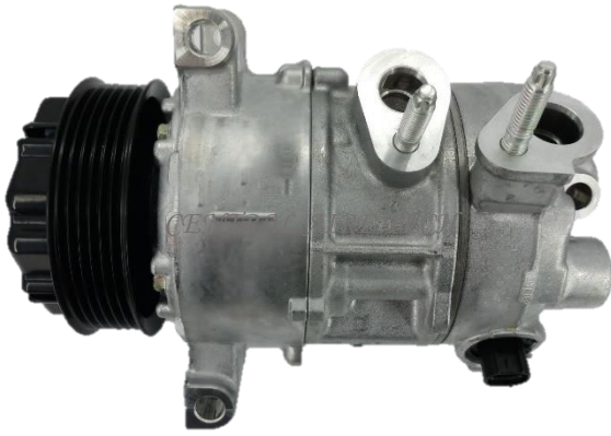
DENSO CAT NO. 12-007 COMPRESSOR TYPE: 5SE12C CAR MODEL: CALIBER 1.8/2.0L YEAR MODEL: 2009 GROOVE: 6PK
