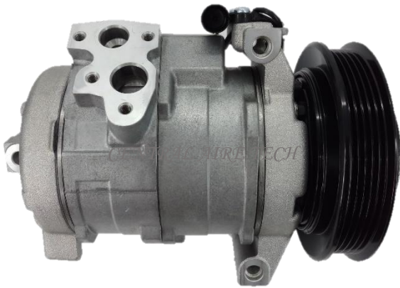
DENSO CAT NO. 29-025 COMPRESSOR TYPE: 10S17C (LSF) CAR MODEL: SPRINTER 3.5L YEAR MODEL: 2009 GROOVE: 5PK
