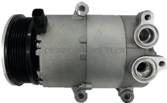
HALLA CAT NO. 14-015 COMPRESSOR TYPE: VS16 CAR MODEL: MONDEO 4 / S-MAX YEAR MODEL: 2012 GROOVE: 6PK
