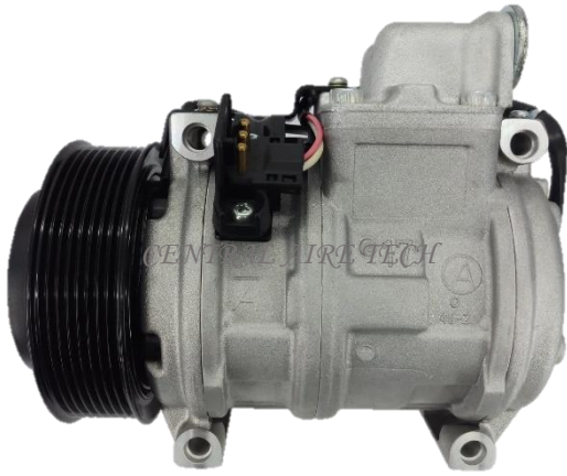
DENSO CAT NO. 29-067 COMPRESSOR TYPE: 10PA17C CAR MODEL: M.BENZ YEAR MODEL: GROOVE: 8PK
