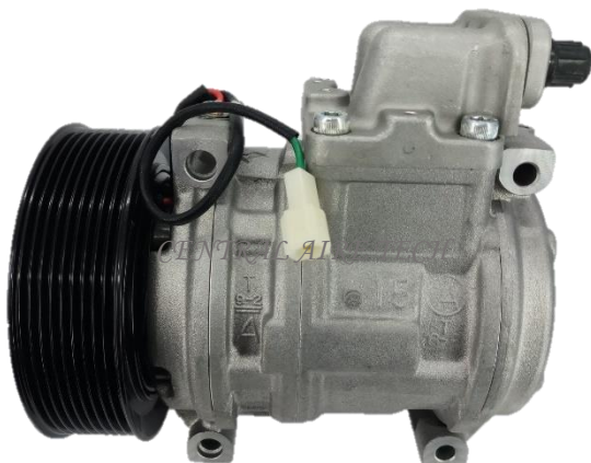
DENSO CAT NO. 29-041 COMPRESSOR TYPE: 10PA15C CAR MODEL: TRUCK YEAR MODEL: GROOVE: 9PK
