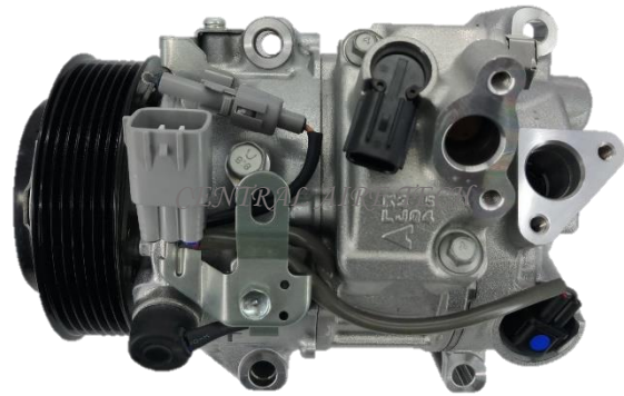
DENSO CAT NO. 27-016 COMPRESSOR TYPE: TSB19C CAR MODEL: GS350 3.5L V6 YEAR MODEL: 2013-2015 GROOVE: 7PK
