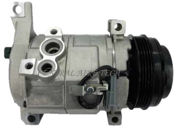
DENSO CAT NO. 08-002 COMPRESSOR TYPE: 10S20F (SENSOR TYPE) CAR MODEL: AVALANCHE 5.3 YEAR MODEL: 2005 GROOVE: 4PK
