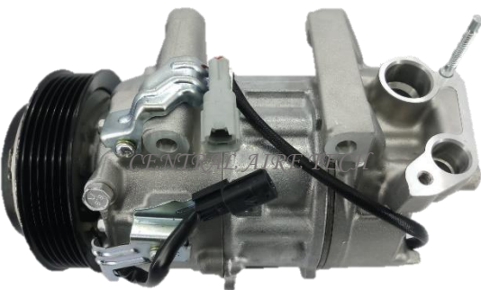
DENSO CAT NO. 32-137 COMPRESSOR TYPE: 6SBH14F CAR MODEL: X-TRAIL QR25/ROGUE 2.5L YEAR MODEL: 2014-2017 GROOVE: 6PK
