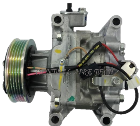
SANDEN CAT NO. 18-070 COMPRESSOR TYPE: STR06 CAR MODEL: BRIO 3851 YEAR MODEL: 2014 GROOVE: 5PK
