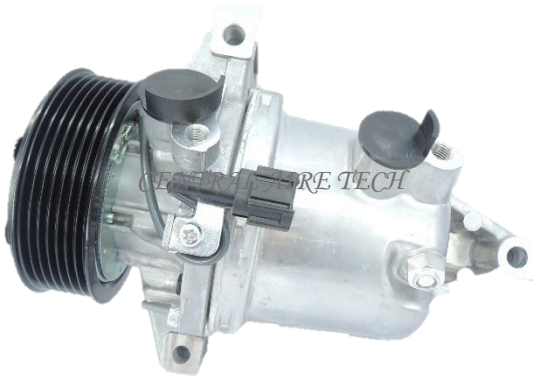
CALSONIC CAT NO. 32-021 COMPRESSOR TYPE: CR08B CAR MODEL: ALMERA 1.5L/JUKE 1.6L YEAR MODEL: 2015 GROOVE: 7PK
