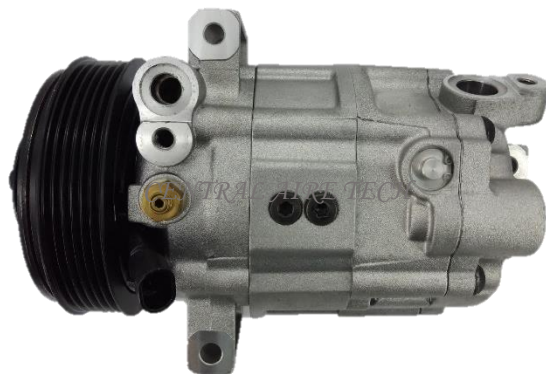
ZEXEL CAT NO. 38-002 COMPRESSOR TYPE: DCV14J CAR MODEL: L300 3.0L GAS YEAR MODEL: 2000-2005 GROOVE: 6PK
