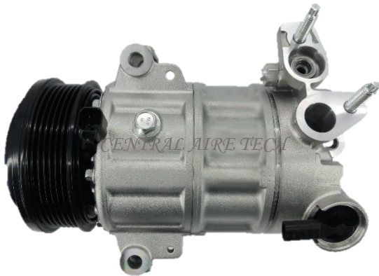
FOMOCO CAT NO. 14-069 COMPRESSOR TYPE: BGDPA CAR MODEL: ECOSPORT TITANIUM 1.0L YEAR MODEL: 2018-2019 GROOVE: 6PK
