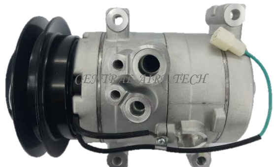
DELPHI CAT NO. 16-006 COMPRESSOR TYPE: CSP15 (RSF) CAR MODEL: JAC (24V) YEAR MODEL: GROOVE: 1B
