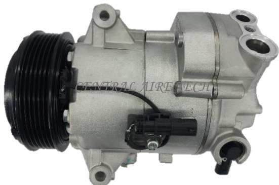
DELPHI CAT NO. 03-023 COMPRESSOR TYPE: 6CVC CAR MODEL: VERANO 2.0 YEAR MODEL: 2012 GROOVE: 6PK
