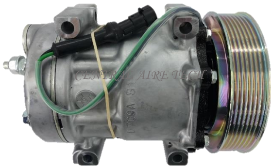
SANDEN CAT NO. 51-001 COMPRESSOR TYPE: SD7H15 (SB REAR) CAR MODEL: TRUCK XF95 YEAR MODEL: 2009 GROOVE: 7PK
