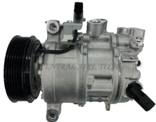
DENSO CAT NO. 01-018 COMPRESSOR TYPE: 6SAS14C CAR MODEL: A6 / S6 YEAR MODEL: 2014 GROOVE: 6PK
