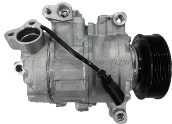
DENSO CAT NO. 45-034 COMPRESSOR TYPE: 6SEU14C CAR MODEL: TOURAGE / AUDI Q7 4L YEAR MODEL: 2007 GROOVE: 6PK
