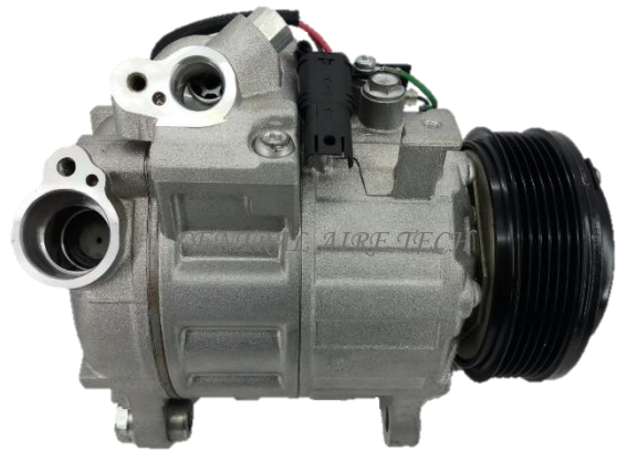
VALEO CAT NO. 02-034 COMPRESSOR TYPE: DCS17EC CAR MODEL: 520i F18 YEAR MODEL: 2008-2011 GROOVE: 6PK
