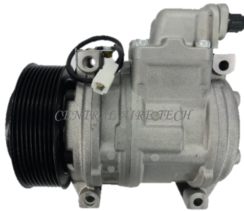
DENSO CAT NO. 29-062 COMPRESSOR TYPE: 10PA15C CAR MODEL: TRUCK 24V YEAR MODEL: GROOVE: 9PK
