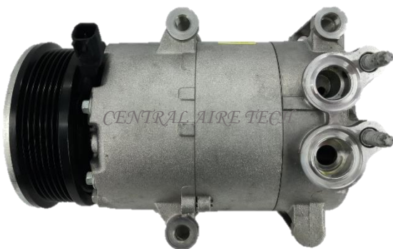
HALLA CAT NO. 14-011 COMPRESSOR TYPE: VS16 CAR MODEL: MONDEO 4 YEAR MODEL: 2012 GROOVE: 6PK
