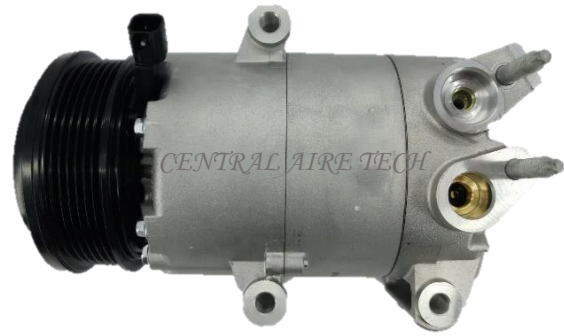
HALLA CAT NO. 14-062 COMPRESSOR TYPE: VS16 CAR MODEL : FOCUS 1.8L YEAR MODEL: 2016 GROOVE: 6PK
