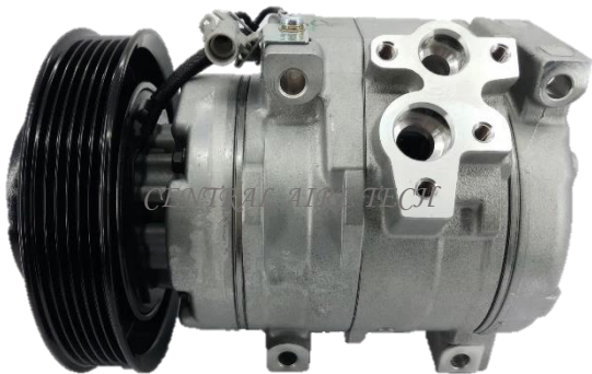
DENSO CAT NO. 44-021 COMPRESSOR TYPE: 10S15L CAR MODEL: ALTIS 1.6L YEAR MODEL: 2002 GROOVE: 6PK
