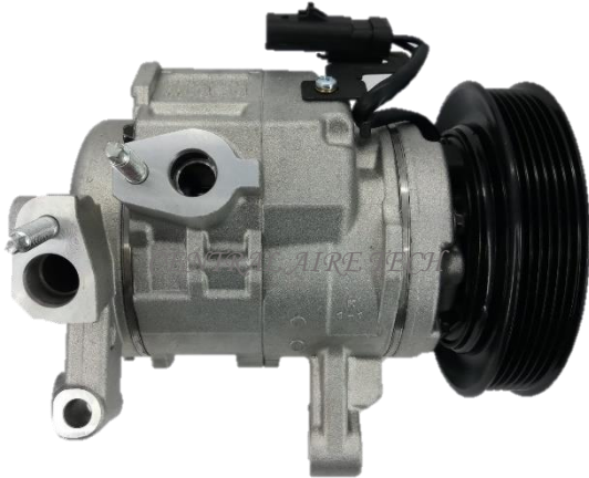
DENSO CAT NO. 12-016 COMPRESSOR TYPE: 10SR17E CAR MODEL: DURANGO YEAR MODEL: 2008-2009 GROOVE: 6PK
