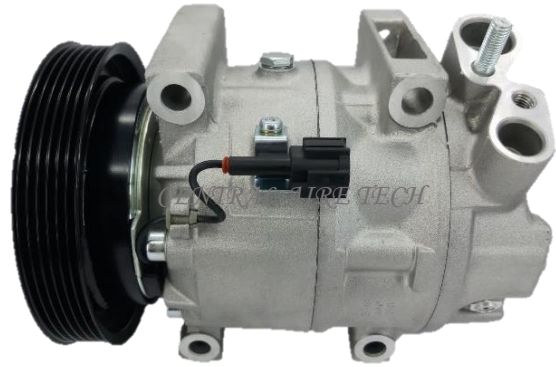
CALSONIC CAT NO. 32-092 COMPRESSOR TYPE: CWV618 CAR MODEL: SERENA 2.5L YEAR MODEL: 2003 GROOVE: 6PK
