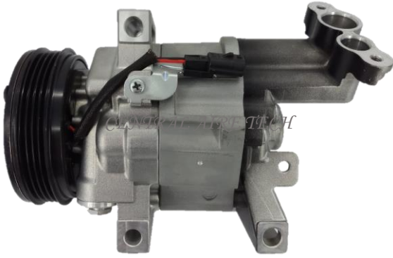
ZEXEL CAT NO. 10-001 COMPRESSOR TYPE: DKV11R (3DM BOTTOM) CAR MODEL: DUSTER YEAR MODEL: GROOVE: 4PK
