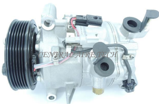
SANDEN CAT NO. 32-071 COMPRESSOR TYPE: PXC14 CAR MODEL: SENTRA/INFINITY Q50 3.7L YEAR MODEL: 2014-2016 GROOVE: 6PK
