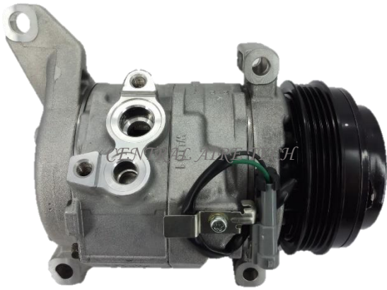
DENSO CAT NO. 04-001 COMPRESSOR TYPE: 10SE18F CAR MODEL: SILVERADO 2.5/3.5/4.8 YEAR MODEL: 2011-2013 GROOVE: 4PK
