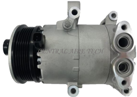
HALLA CAT NO. 14-008 COMPRESSOR TYPE: VS16 CAR MODEL: FOCUS 1.6L YEAR MODEL: 2005-2008 GROOVE: 6PK
