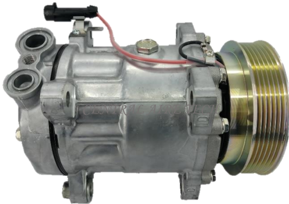
DENSO CAT NO. 65-003 COMPRESSOR TYPE: SD7V16 (VUA) CAR MODEL: 166/LANCIA 2.0 YEAR MODEL: 1998 GROOVE: 6PK
