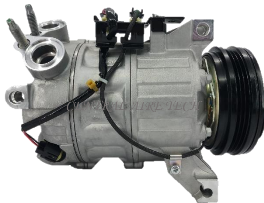
VALEO CAT NO. 46-016 COMPRESSOR TYPE: DCS17EC (LSF) CAR MODEL: S80/S60/V7 YEAR MODEL: 2011-2013 GROOVE: 3PK
