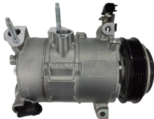
FOMOCO CAT NO. 14-006 COMPRESSOR TYPE: 6SBH14C CMDL: MUSTANG ECOBOOST L4 4.3L GAS YEAR MODEL: 2015-2020 GROOVE: 4PK
