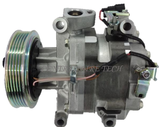
DENSO CAT NO. 18-047 COMPRESSOR TYPE: STR08 CAR MODEL: JAZZ / CITY 1.3L YEAR MODEL: 2014 GROOVE: 5PK
