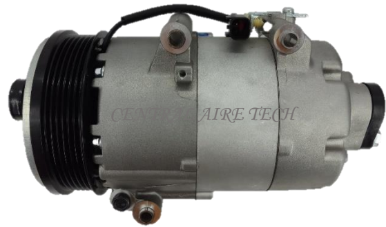
HALLA CAT NO. 14-010 COMPRESSOR TYPE: VS16 CAR MODEL: FOCUS 2.0L YEAR MODEL: 2008 GROOVE: 6PK
