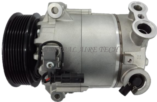
DELPHI CAT NO. 03-021 COMPRESSOR TYPE: CVCE CAR MODEL: LACROSSE 2.4L GAS YEAR MODEL: 2012-2016 GROOVE: 7PK
