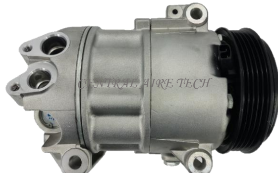
DELPHI CAT NO. 13-018 COMPRESSOR TYPE: 6CVC CAR MODEL: 500L/124 SPIDER 1.4L YEAR MODEL: 2017-2020 GROOVE: 5PK
