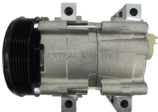
HALLA CAT NO. 14-083 COMPRESSOR TYPE: FS10 CAR MODEL: EXPLORER 4.0L YEAR MODEL: 1999 GROOVE: 6PK
