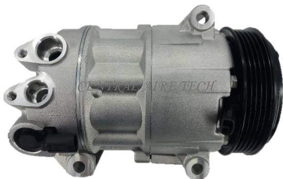
DELPHI CAT NO. 13-017 COMPRESSOR TYPE: 6CVC CAR MODEL: 500X/JEEP RENEGADE 1.4L YEAR MODEL: 2016-2018 GROOVE: 5PK
