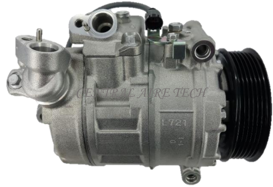
DENSO CAT NO. 02-008 COMPRESSOR TYPE: 7SEU17C CAR MODEL: E65 4.8 YEAR MODEL: 2005 GROOVE: 6PK
