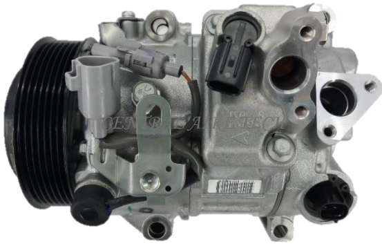
DENSO CAT NO. 27-013 COMPRESSOR TYPE: TSB17C CAR MODEL: ES350 YEAR MODEL: 2016 GROOVE: 7PK
