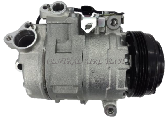
DENSO CAT NO. 02-044 COMPRESSOR TYPE: 7SBU17C CAR MODEL: E60 / E61 / E63 / E64 YEAR MODEL: 2005-2010 GROOVE: 4PK
