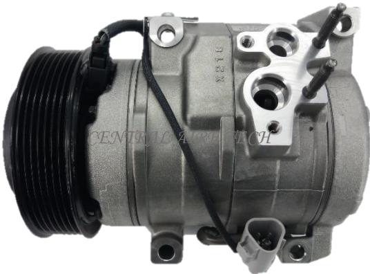
DENSO CAT NO. 44-140 COMPRESSOR TYPE: 10S17C CAR MODEL: NOAH YEAR MODEL: GROOVE: 7PK
