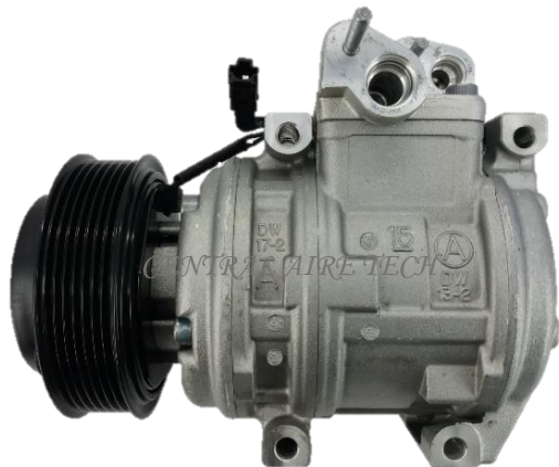
DOOWON CAT NO. 24-017 COMPRESSOR TYPE: 10PA15L CAR MODEL: SORENTO 2.5L DSL YEAR MODEL: 2008 GROOVE: 7PK
