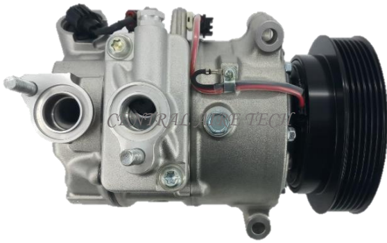
SANDEN CAT NO. 46-013 COMPRESSOR TYPE: PXC16 CAR MODEL: S80 YEAR MODEL: 2011 GROOVE: 6PK
